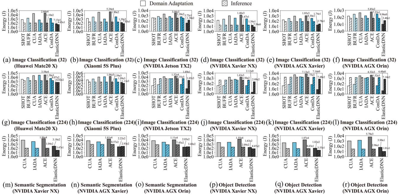
Fig. 8. Average energy consumption in each domain on heterogeneous devices.
