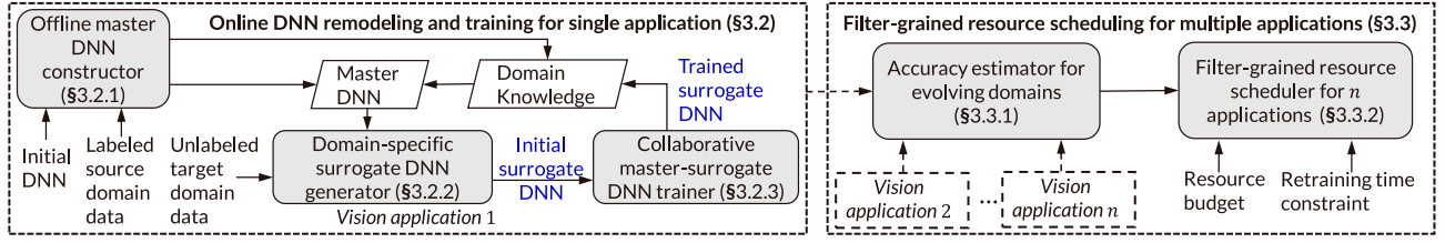
Fig. 2. ElasticDNN overview.
