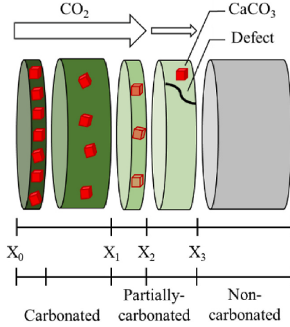
Fig. 8. Illustration of the generated \text{CaCO}_3 along different zones after carbonation of the early-hydration-age cement paste.
