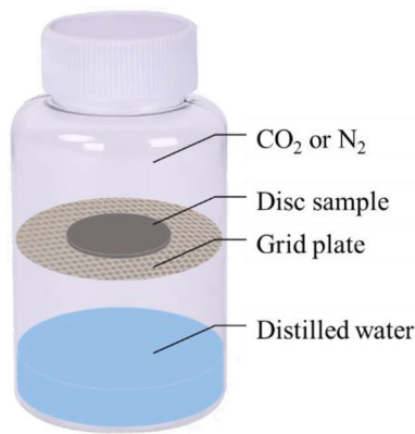
Fig. 2. Schematic diagram of the reaction device for carbonation ( \text{CO}_2 ) or carbonation free ( \text{N}_2 ) as the reference.
