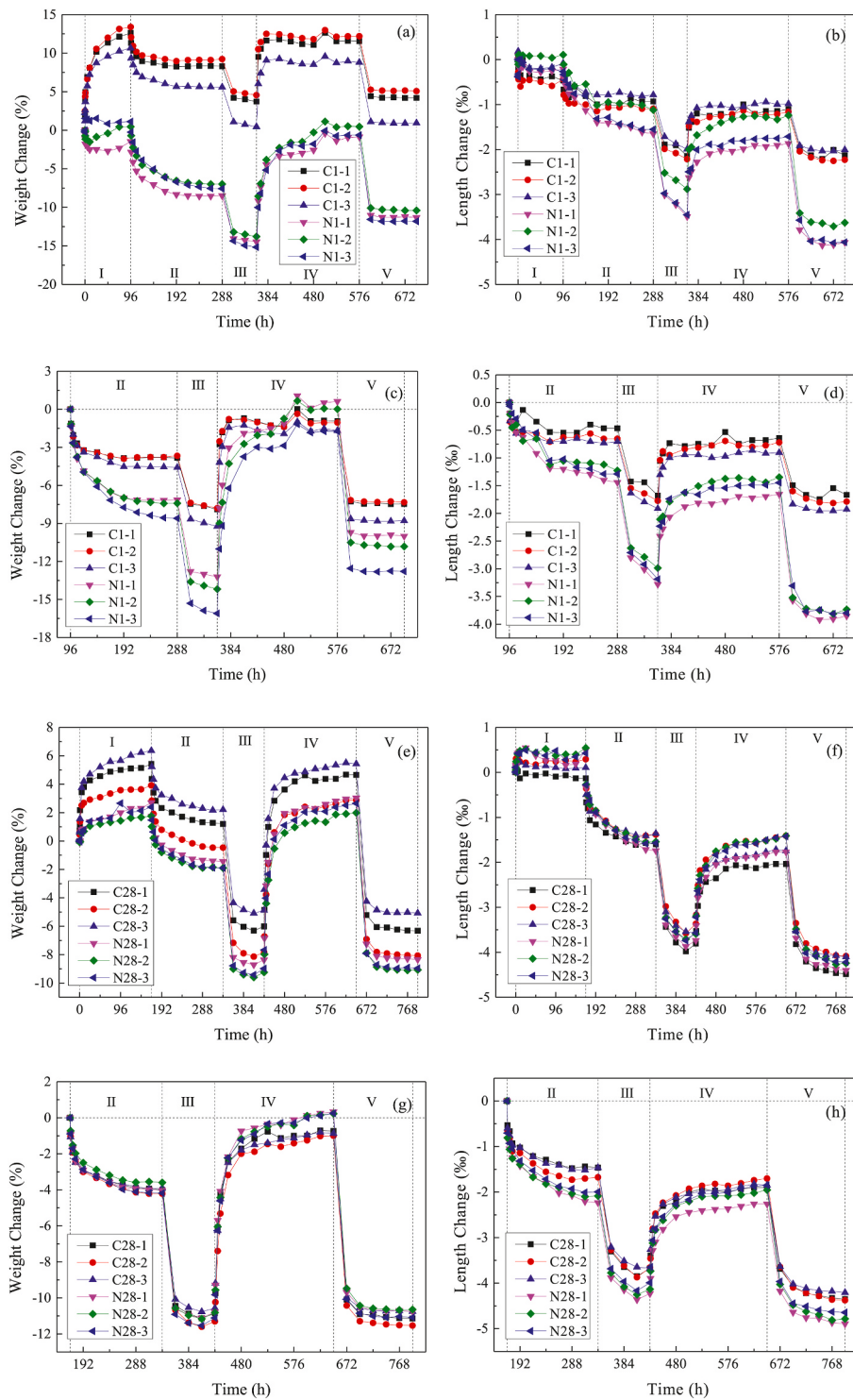
Fig. 10. Weight and length changes of disc samples carbonated at hydration time of 1 d and 28 d during the whole and parts of 5 stages of experimental process. (a)–(d): 1 d; (e)–(h): 28 d. (a), (c), (e), and (g): weight changes; (b), (d), (f), and (h): length changes. (a), (b), (e), and (f): start at carbonation stage; (c), (d), (g), and (h): start at drying stage.
