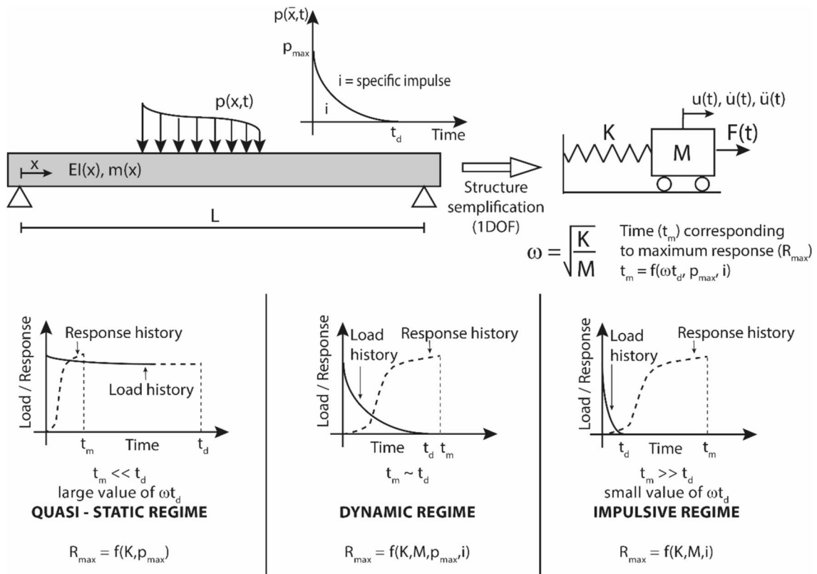
Fig. 1 Structural response regimes for a structure simplified with a Single Degree of Freedom System
