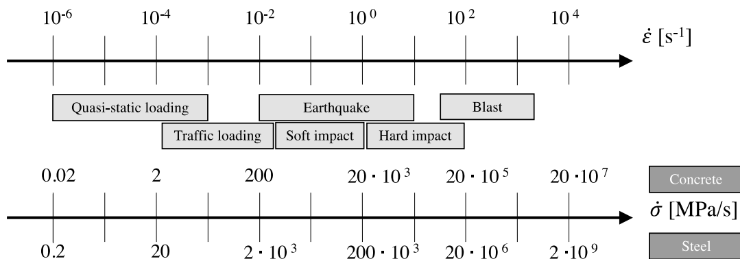
Fig. 2 Elastic strain-rates for different loading velocities [17, 31] and correspondent stress-rates. Note: in the figure elastic modulus for concrete is considered equal to 20 GPa while 200 GPa for steel
