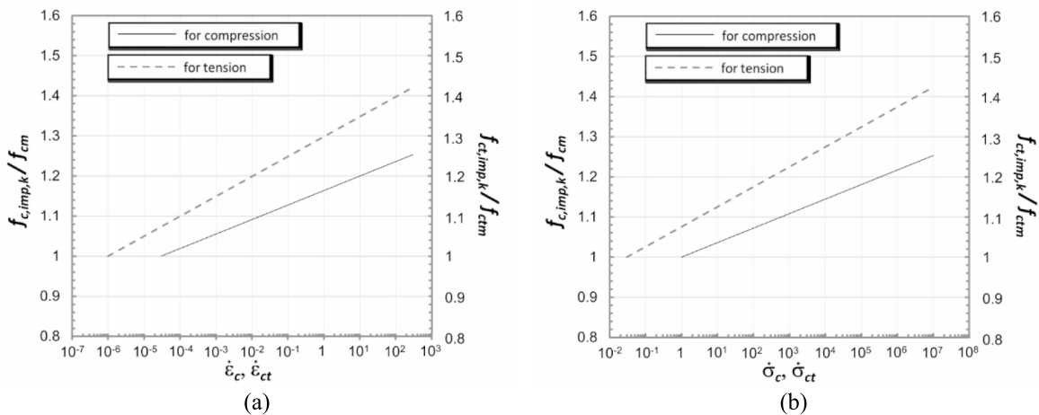
Fig. 3 Effect on compressive and tensile strength of concrete of a strain-rate and b stress-rate
