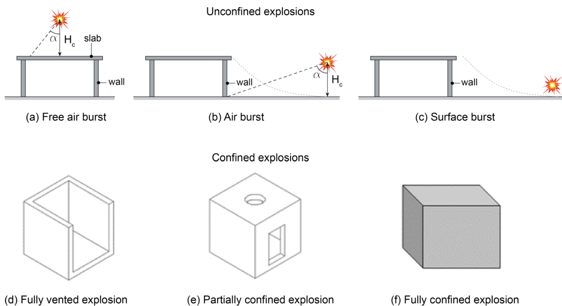
Fig. 6 Blast-loading categories
