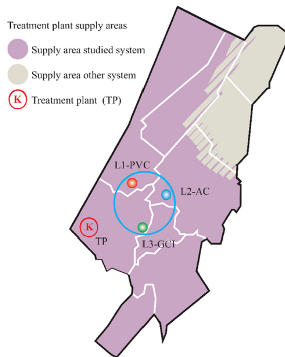
Fig. 1. Layout of the distribution area and sampling locations. L1, PVC-U pipe (1978, 42 years old); L2, AC pipe (1962, 58 years old); L3, GCI pipe (1970, 50 years old).
