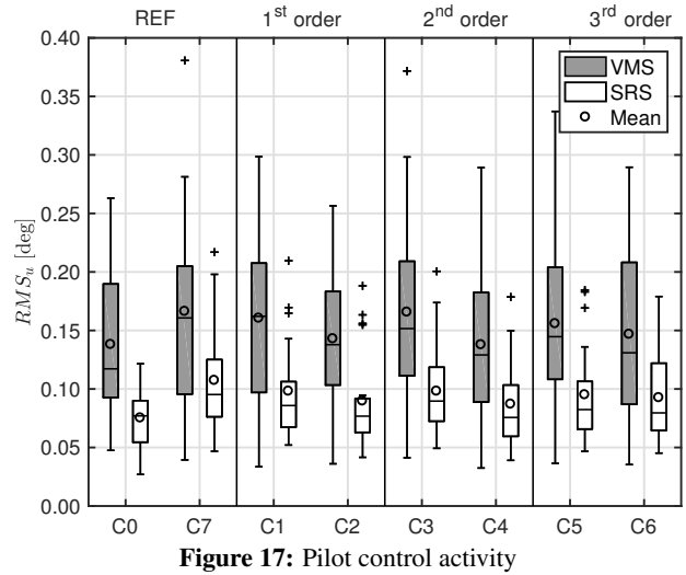
Figure 17: Pilot control activity
