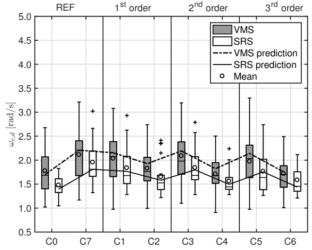
Figure 28: Open-loop disturbance crossover frequency \omega_{c,d}
