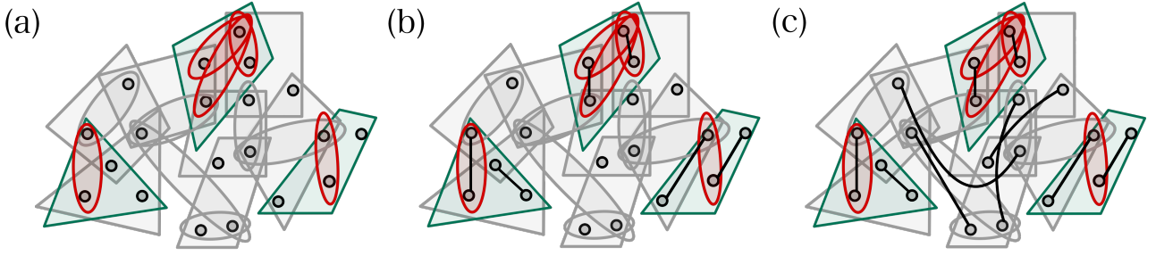
Figure 3: Example of the construction from the proof of Lemma 20. (a) The q -local set of interactions \mathcal{I} ( q = 4 ). Highlighted in green is diffuse and strictly q' -local \mathcal{T}' ( q' = 4 ), in red are the interactions in \text{Sup}(\mathcal{T}') with weight less than q' , in grey are the rest of interactions in \mathcal{I} . The goal is to create a matching M consistent with green-colored terms, inconsistent with grey-colored terms, and with no guaranteed relation to the red-colored terms. (b) Matching M' on \text{Sup}(\mathcal{T}') , consistent with \mathcal{T}' by construction. Ensuring inconsistency with all red-colored terms is in general impossible. For example, consider the three overlapping red-colored terms at the top center. (c) Completing M = M' \cup M'' with a matching M'' on [2n] \setminus \text{Sup}(\mathcal{T}') , ensuring inconsistency with all grey-colored terms. For this, the vertices are matched only if they belong to different interactions.
