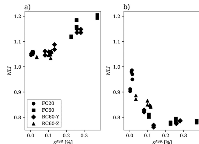
Fig. 24. NLI against expansion for a) the first load cycle, and b) as the average of the last four cycles.
