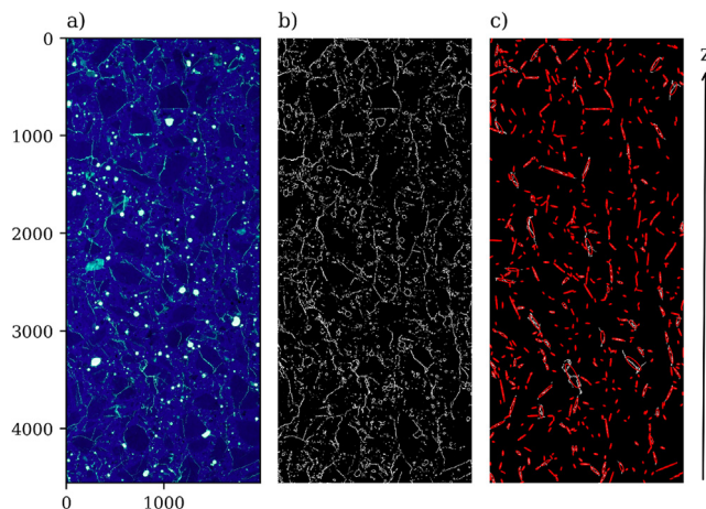
Fig. 21. Petrographic examination results of RC60-3b with a) cropped original image, b) binary image, and c) final processed image.
