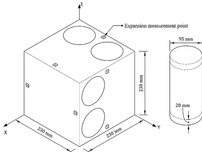
Fig. 3. Two cores were drilled from the restrained cubes in two directions (Y and Z). The cubes were cast along the X-axis; the Z-axis is the restrained direction.
