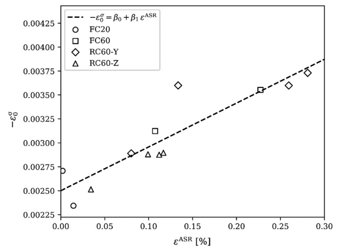
Fig. 18. Peak compressive strain against ASR expansion. The coefficients in the regression function are \beta_0 = 0.0025 and \beta_1 = 0.45 . R^2 = 0.82 .
