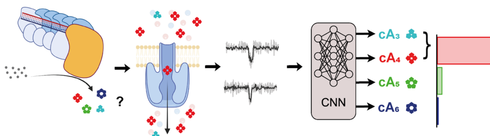
Figure 6. Nanopore-CNN pipeline for the identification of single second messengers from type III CRISPR-Cas. Biological cOAs of unknown stoichiometry, produced by CRISPR type III-A and III-B complexes, are detected one by one in nanopore experiments. Single-molecule events extracted from the nanopore reads are then identified by a pretrained CNN, yielding the stoichiometric composition of the biological cOA samples.
