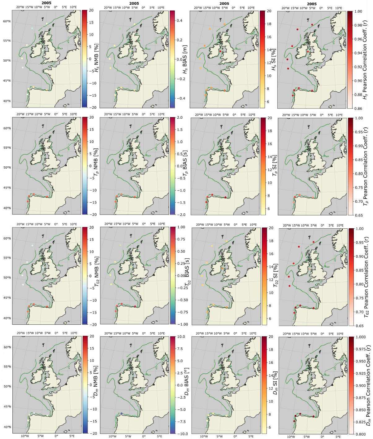
Figure 9: Model performance indicators obtained comparing with buoy data for (a) H_s , (b) T_p , (c) T_{02} and (d) D_m . Results for validation year 2005 using TUD-165.
