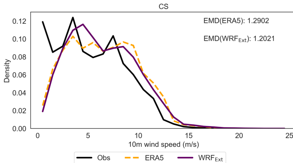
Figure 29: Same as Figure 27, but at the CS location.
