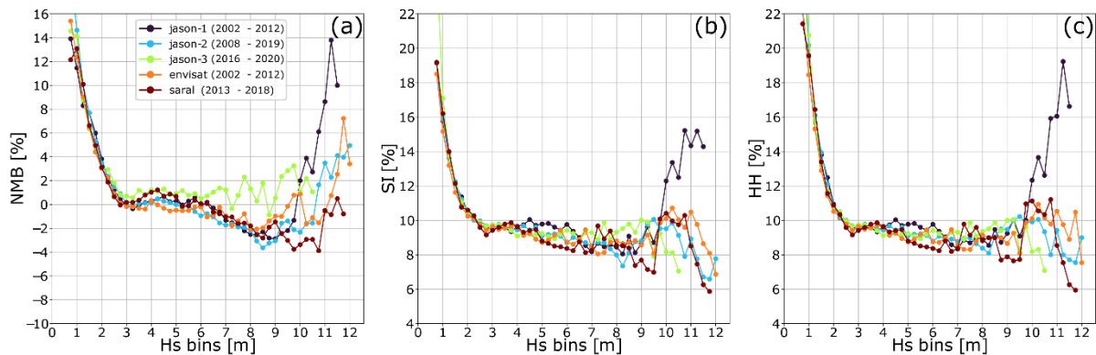
Figure 8: Hindcast validation obtained with different altimeters' (full) mission time windows. (a) H_s normalized mean bias (NMB), (b) scatter index (SI) and (c) Hanna Heinhold index (HH).
