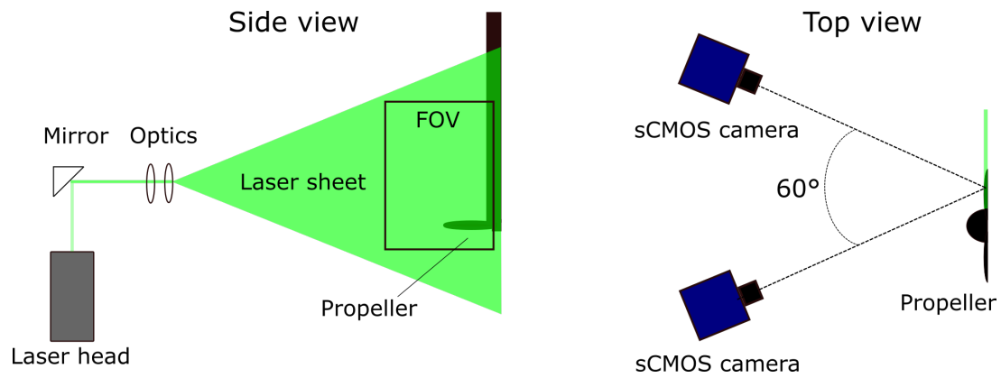
Figure 4. Stereoscopic PIV setup: (left) side view, (right) top view.
