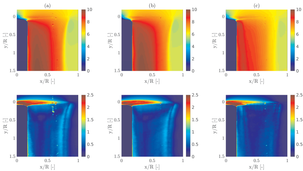
Figure 11. Mean velocity (top) and rms velocity (bottom) at v = 6 \text{ m/s} and \Omega = 5000 \text{ RPM} . (a) represents the baseline propeller, (b) the b_1h_2 propeller and (c) the b_3h_3 propeller.
