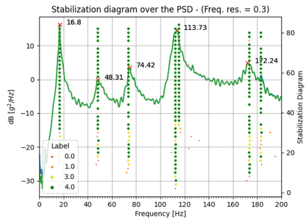
Fig. 15. Damage level 2 PCB equipment, results in frequency spectrum
