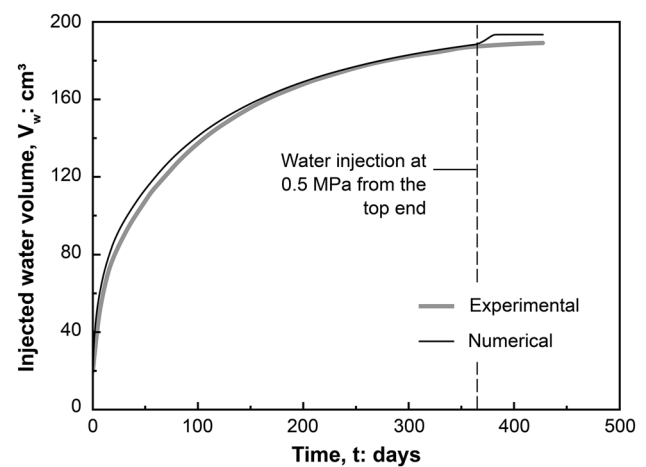
Fig. 4 Water volume injected from the bottom end. Comparison between experimental data and model predictions
