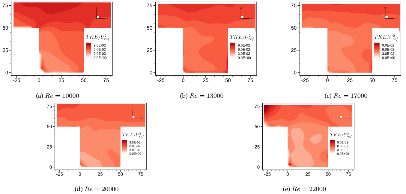
Figure 12. Contour plots of Turbulence Kinetic Energy at y/L = 0.3
