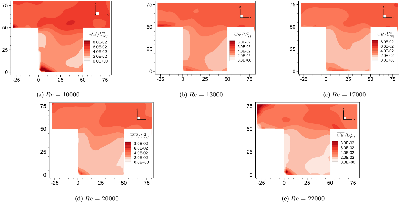
Figure 11. Contour plots of Reynolds stress \overline{u'u'} at y/L = 0.3
