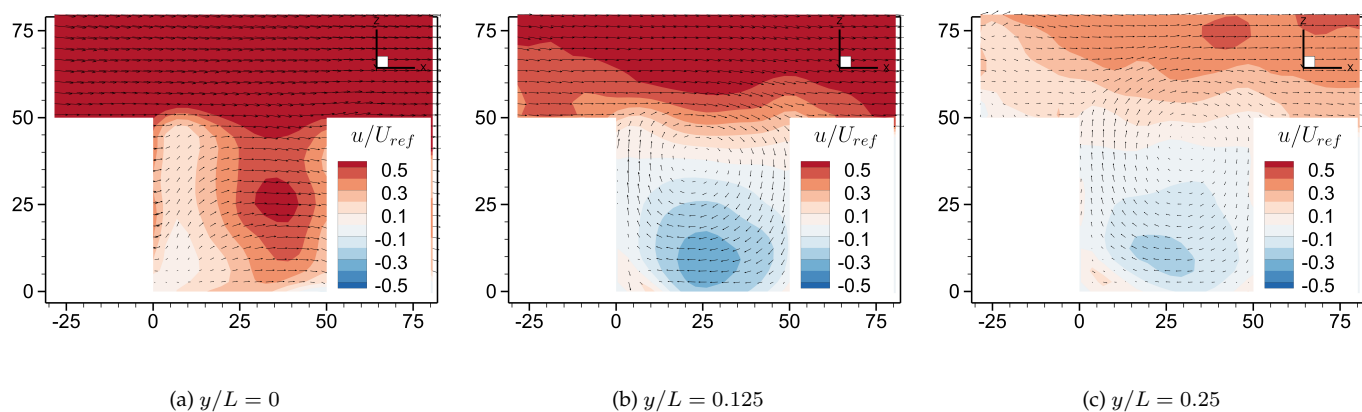
Figure 4. Streamwise Velocity
