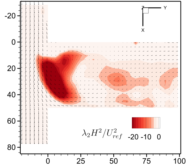
Figure 7. \lambda_2 contours at z/H = 0.5 showing a stable vertical vortex
