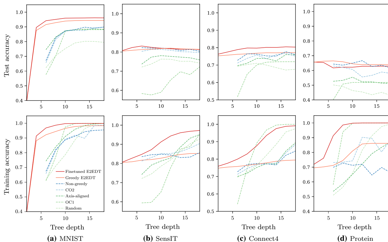
Fig. 2 Accuracy on test and training sets of various optimization methods for deterministic oblique decision trees. For of our proposed approach, we show results with Greedy initialization only (solid, light red line), and after being Finetuned (solid, dark red line). The results of
