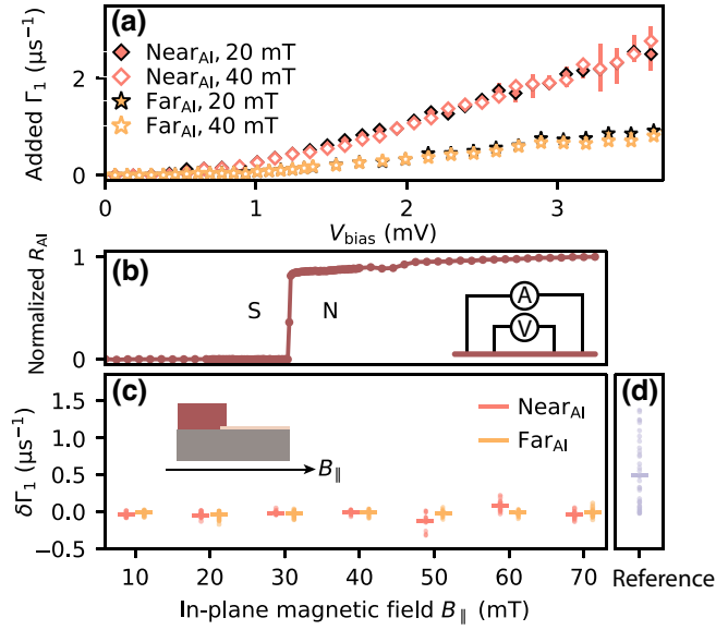
FIG. 4. The magnetic field independence of the added-qubit-loss. (a) The added \Gamma_1 as a function of V_{\text{bias}} for the two qubits with an aluminum ground plane at magnetic fields B_{\parallel} of 20 and 40 mT applied in the plane of the chip [cf. (c), inset]. (b) The four-point measurement of the normalized aluminum film resistance R_{\text{Al}} as a function of B_{\parallel} . The “A” denotes a current meter and “V” denotes a voltmeter. (c) A scatter plot showing the differences between the V_{\text{bias}} dependence of \Gamma_1 at zero and elevated B_{\parallel} for the two qubits with an aluminum ground plane. Each data point represents the difference in rates \delta\Gamma_1 evaluated at equal V_{\text{bias}} . The horizontal line indicates the mean of \delta\Gamma_1 over all V_{\text{bias}} . The inset shows the direction of the applied magnetic field with respect to the cross section of the chip. (d) The same type of plot as (c) but showing the difference between the Near Al and Near Nb-Ti-N qubits at zero applied magnetic field [data shown in Fig. 2(d)]. This serves as a reference for the data in (c).
