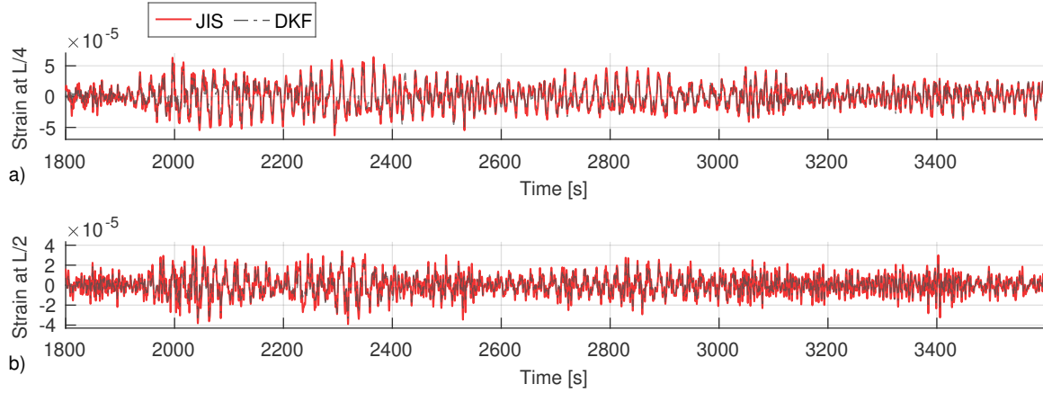
Fig. 16 Estimated strain at the (a) quarter-span, and (b) mid-span for the period t \in [1800, 3600] s
