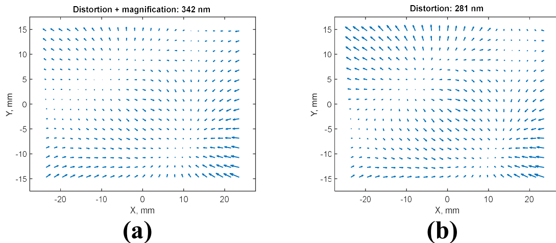
Figure 6. Distortion + magnification (a) and pure distortion (b) in Zoom 2 configuration, measured in a scanning test.
