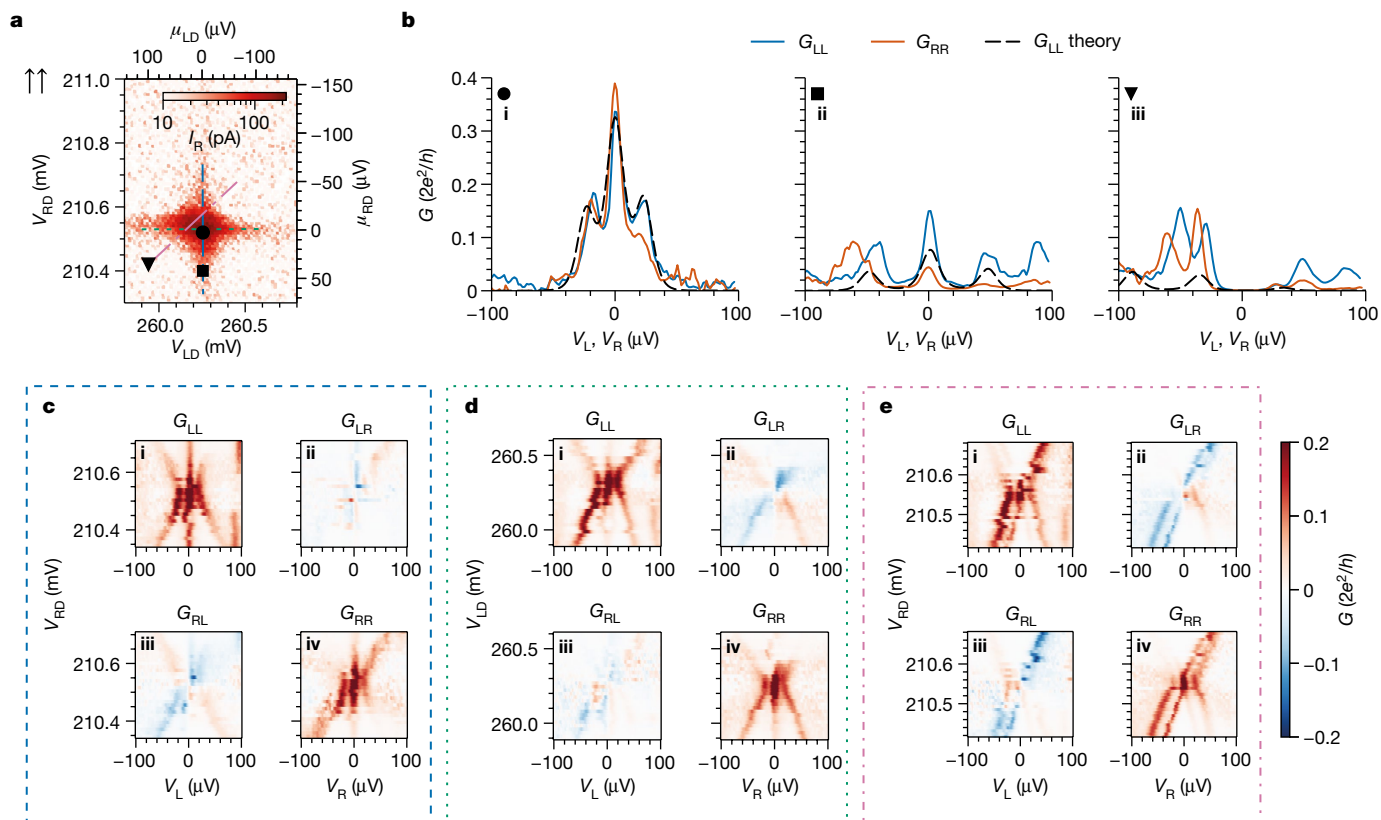
Fig. 3 | Conductance spectroscopy at the t = \Delta sweet spot for the \uparrow\uparrow spin configuration. a , I_R versus V_{LD} and V_{RD} under V_L = 0 and V_R = 10 \mu\text{V} . The spectra in panel b are taken at values of V_{LD} and V_{RD} marked by corresponding symbols. The gate versus bias sweeps are taken along the dashed, dotted and dashed-dotted lines in panels c , d and e , respectively. Data are taken with fixed V_{PG} = 215.1 \text{ mV} . b , Spectra taken under the values of V_{LD} and V_{RD} marked in panel a . The dashed lines are theoretical curves calculated with t = \Delta = 12 \mu\text{eV} ,
