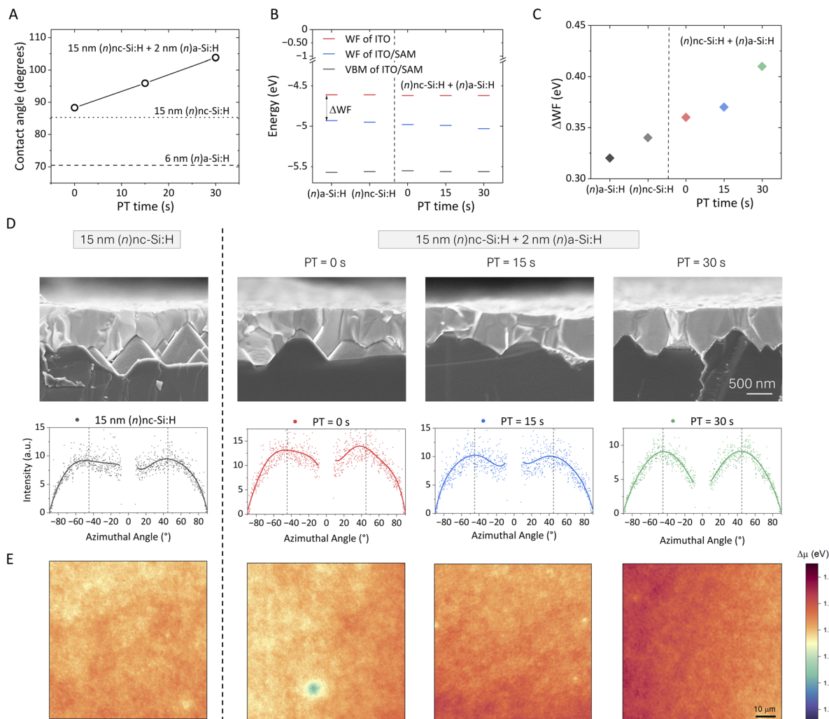
Fig. 3 (A) Contact angle values after HTL-SAM deposition on textured c -Si wafers featuring various plasma treatment (PT) durations on ( n )nc-Si:H layers with 10-nm-thick ITO. The dashed lines in the plot represent the contact angles of samples with 6-nm-thick ( n )a-Si:H and 15-nm-thick ( n )nc-Si:H layers. (B) Valence band maximum (VBM) and WF values, and (C) \Delta WF of ( n )-layer/ITO/SAM (stack) with various plasma treatment durations before and after SAM deposition. (D) Cross-sectional SEM micrographs and azimuthally integrated intensity of the (100) reflection from GIWAXS measurements (Fig. S20). (E) QFLS ( \Delta\mu ) images of perovskite films deposited on different ( n )-layer/ITO/SAM stacks without and with plasma treatment. The SEM micrograph of the sample featuring the ( n )a-Si:H layer is shown in Fig. S21.
