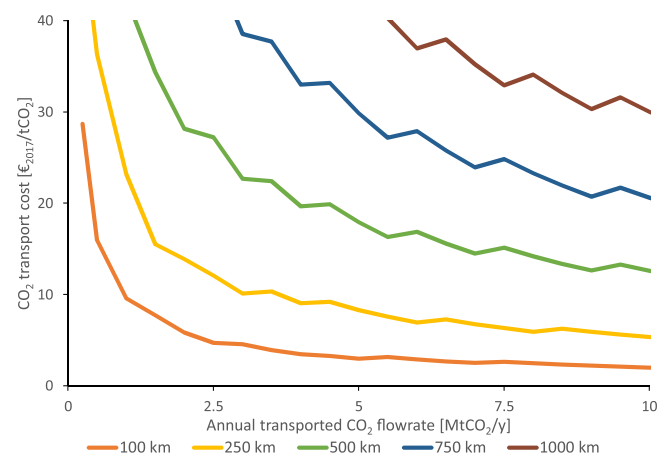
Fig. 10. CO 2 transport cost via offshore pipeline in function of the annual transported CO 2 flowrate for different transport distances.
