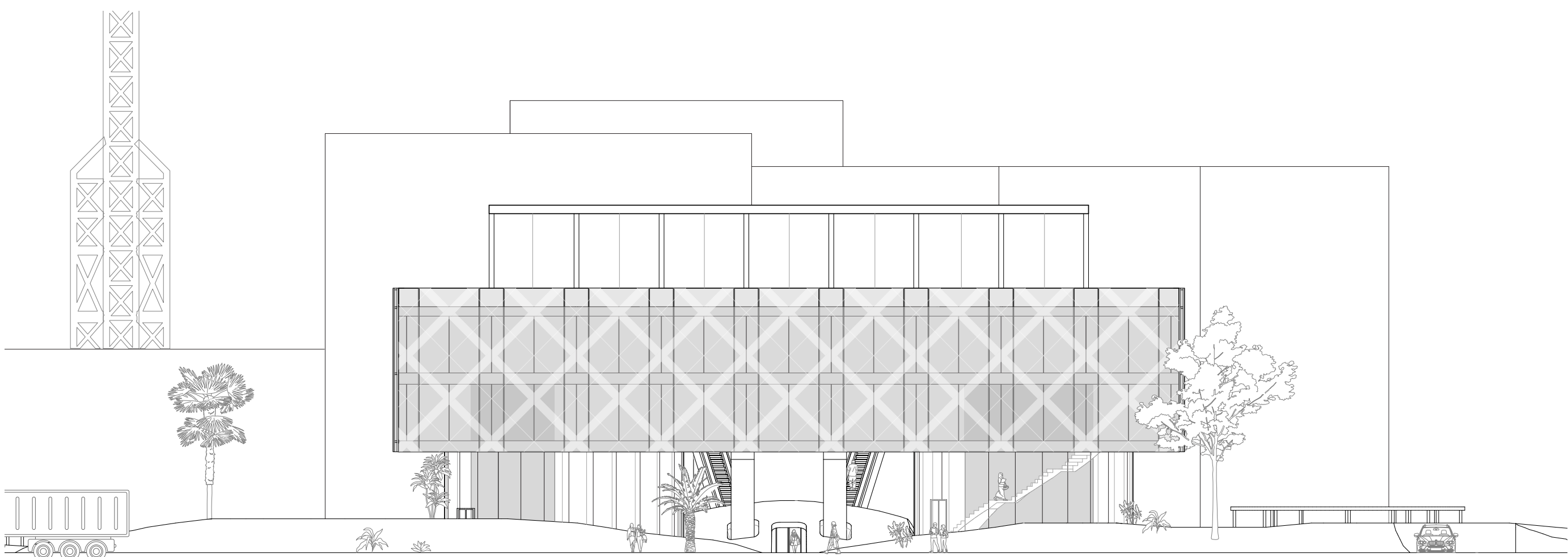
SOUTH ELEVATION
