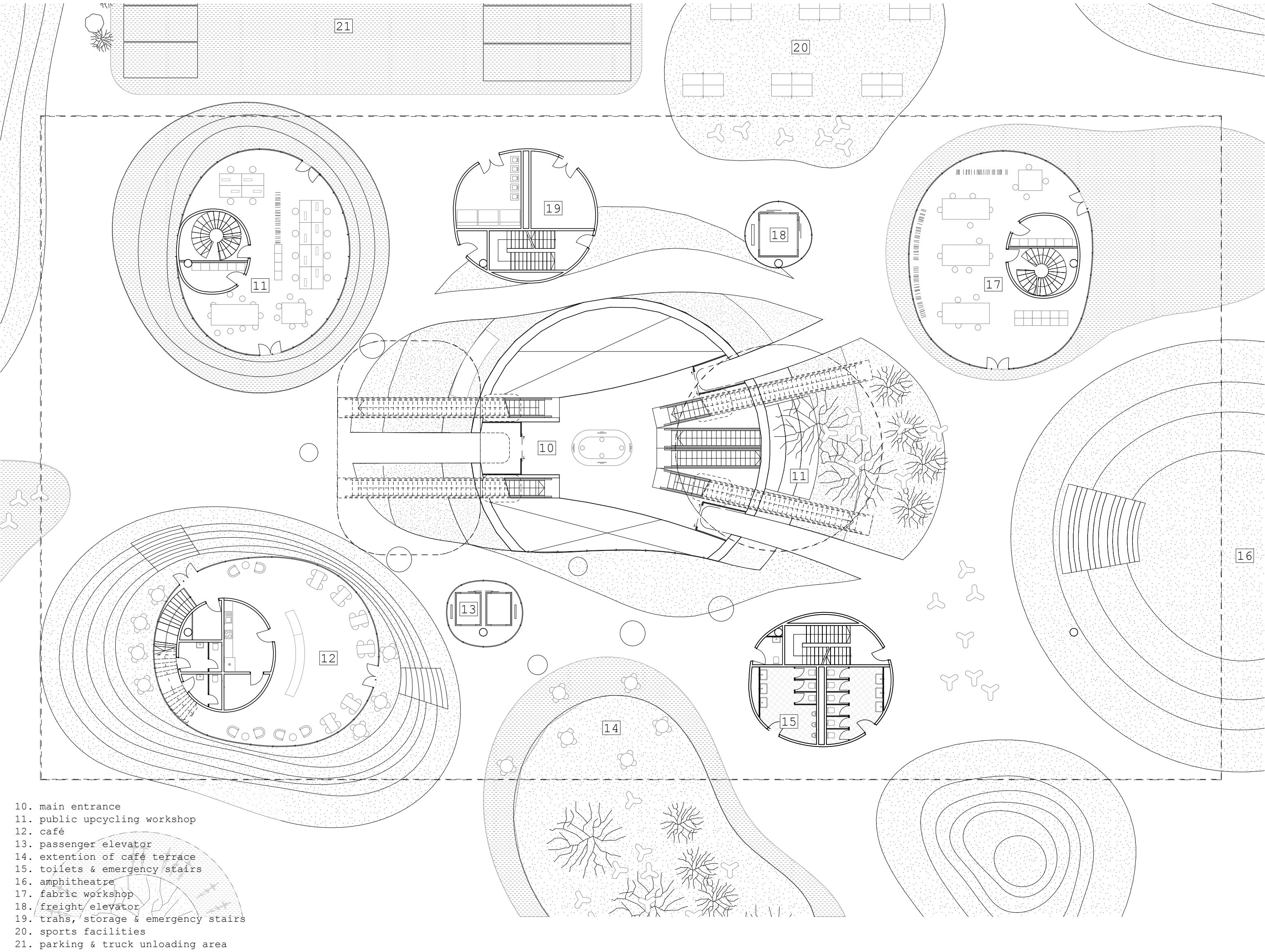
GROUND FLOOR
