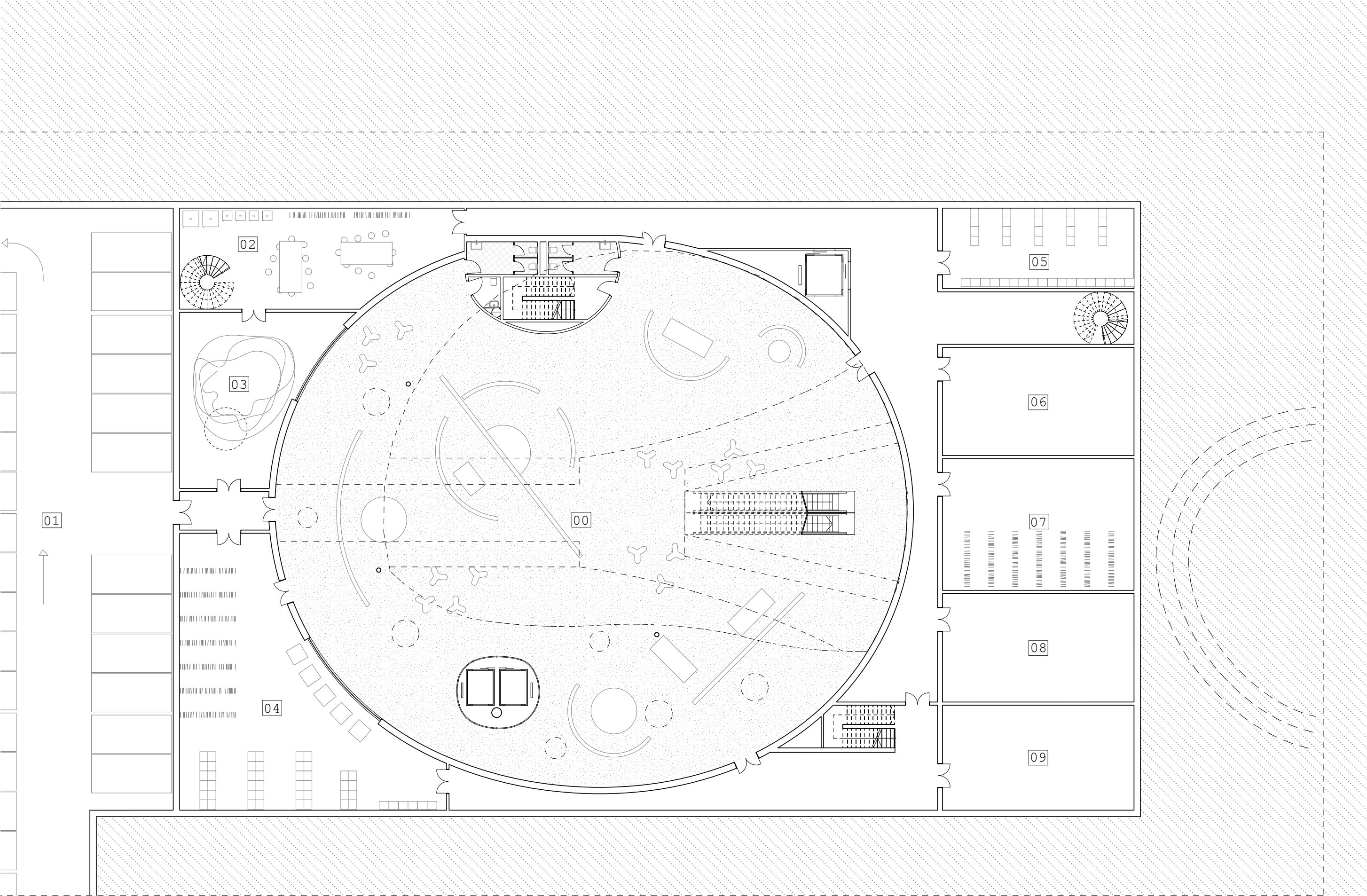
UNDERGROUND FLOOR
