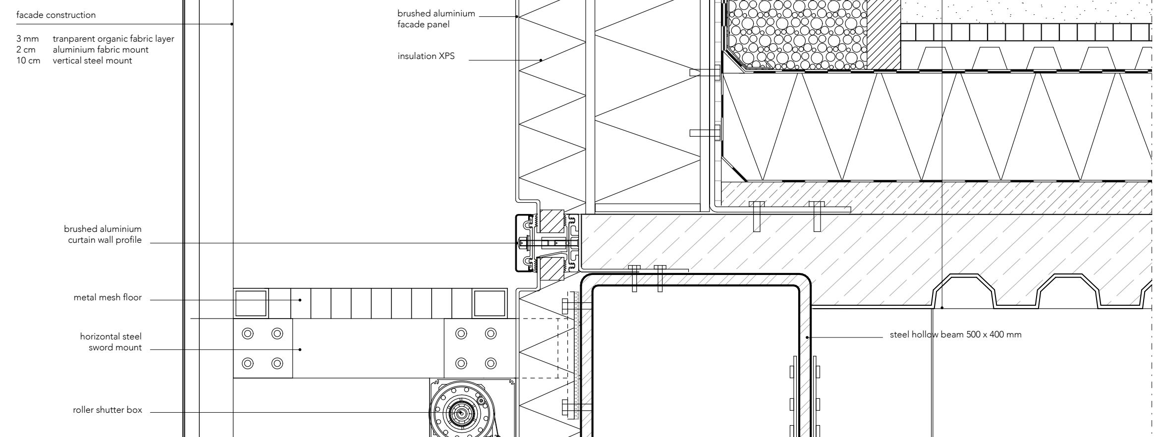
DETAIL 2
