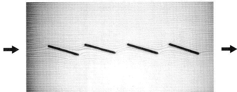
Fig. 7 Four left-stepping cracks arrays. This pictures illustrates the sensitivity of crack's interaction to the slight changes of the geometry of en échelon cracks (compare also with figure 4a).
