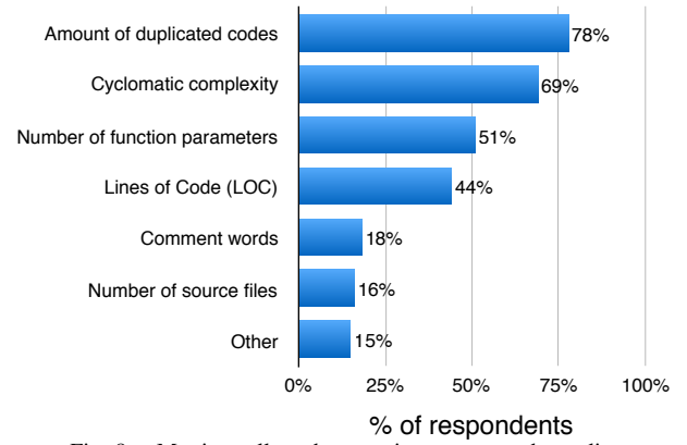
Fig. 8. Metrics collected to monitor source code quality.
