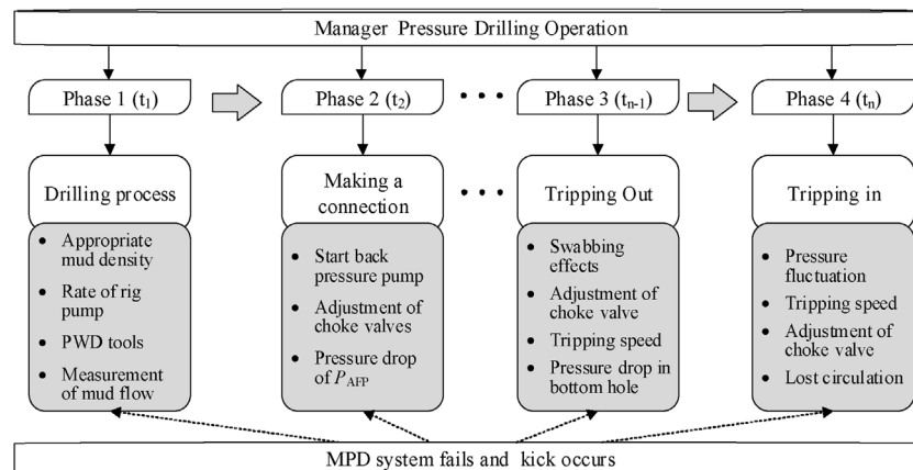
Fig. 6. The managed pressure drilling phases.
