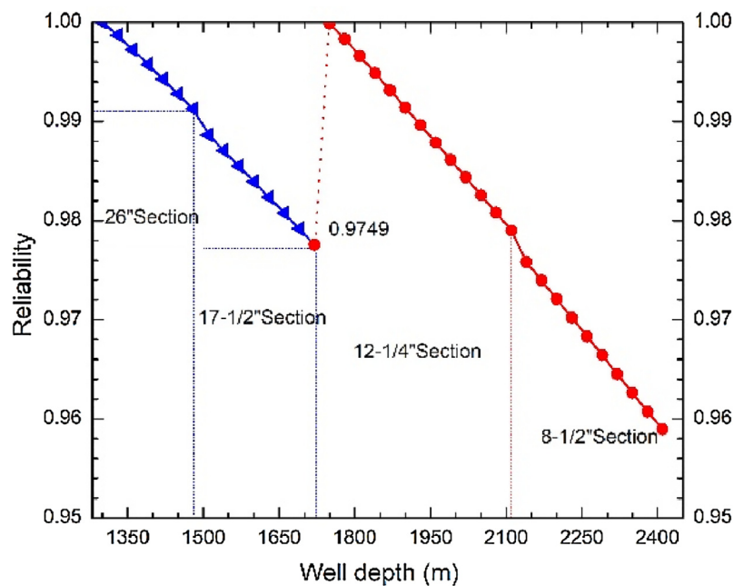
Fig. 15. Updated reliability of drilling cycle for the MPD system.
