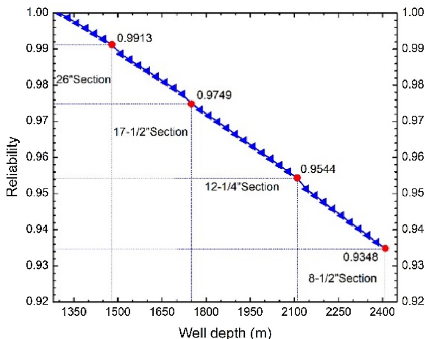
Fig. 13. Dynamic reliability of drilling cycle for the MPD system.
