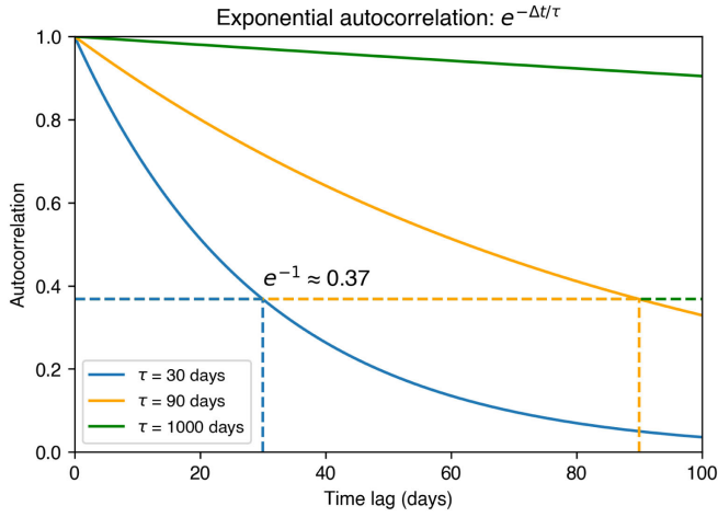
Fig. 2. Exponential autocorrelation of the instantaneous velocity as a function of \Delta t for decorrelation times ( \tau ) of 30, 90, and 1000 days. Notably, the correlation reaches e^{-1} \approx 0.37 when \Delta t = \tau .
