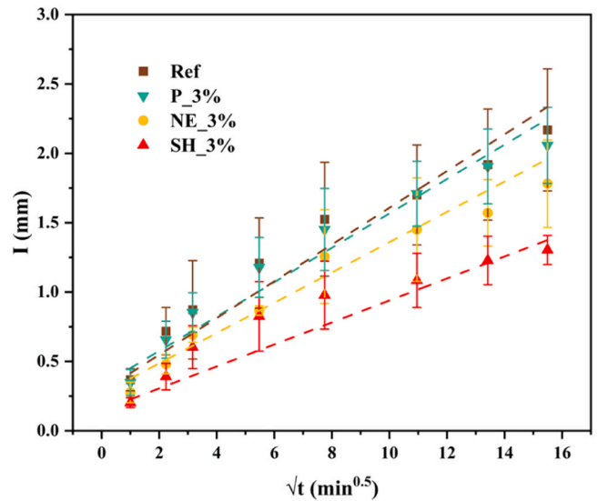
Fig. 18. Cumulative water absorption of the cracked mortar specimens before and after the healing of cracks.
