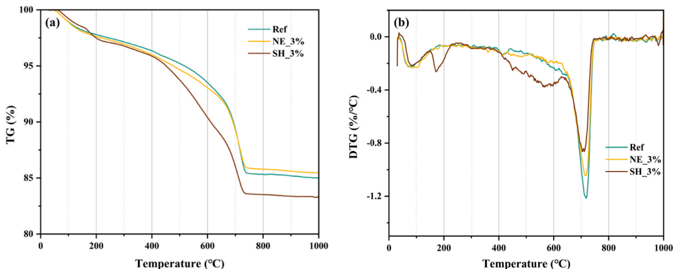
Fig. 21. (a) TG and (b) DTG of the healing products developed in specimens stored under water.
