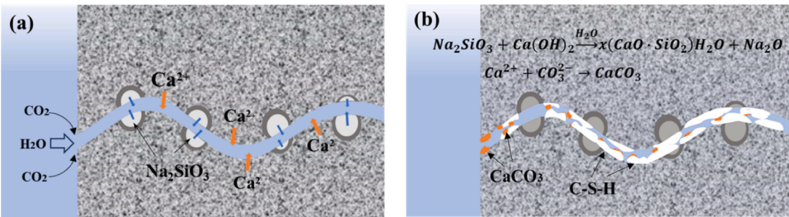
Fig. 24. Schematic diagram of the self-healing process with SH-CS. (a) Cracking in mortar results in the release of Na 2 SiO 3 from the SH-CS; (b) reaction between Ca 2+ with SiO 3 2- and CO 3 2- leads to the precipitation of CaCO 3 and C-S-H gel in the cracking area.
