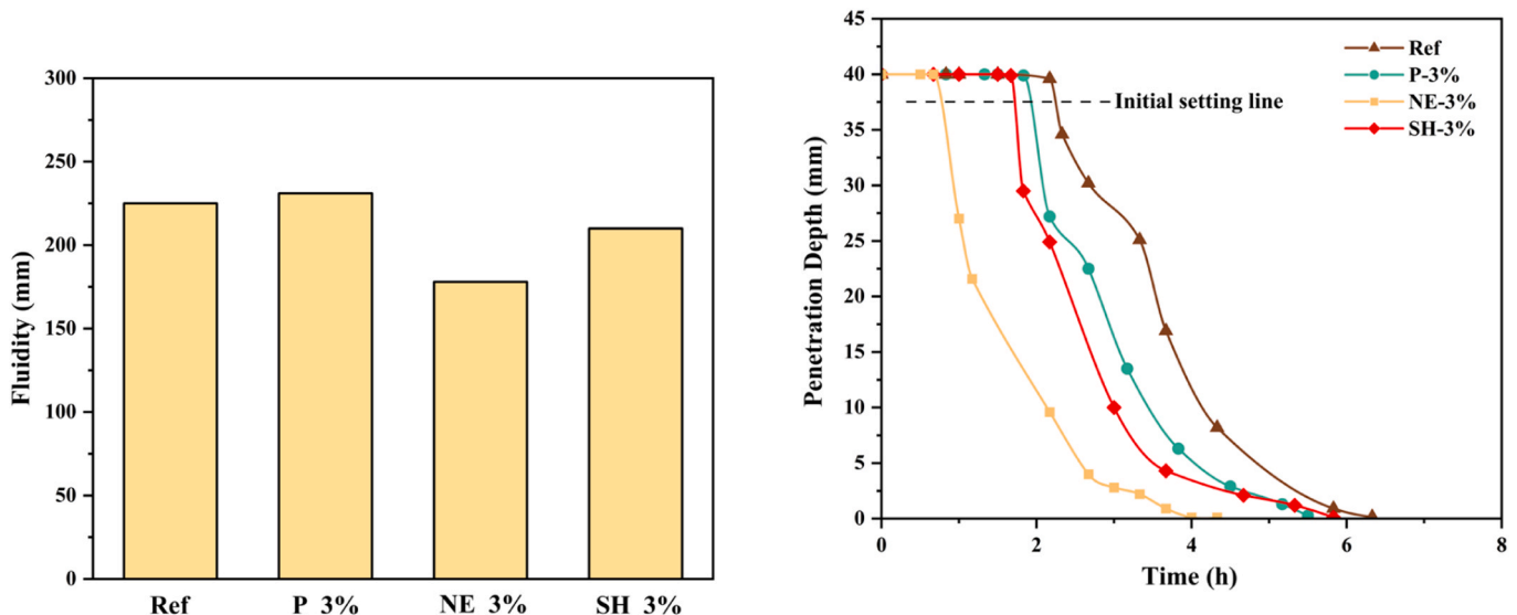
Fig. 8. Effect of different aggregates incorporation on the setting time of mortar.
