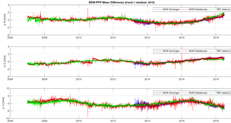
Figure 7.3: Average trend differences between the BSW and PPP solutions for the NAM monitoring and reference stations for the period 2007.0 - 2018.6 : SUM_TREND+RESIDUAL_BSW-PPP . The colored lines are time series of daily averages for respectively the NAM monitoring stations in the Groningen area, monitoring stations in the Waddenzee area and the NAM reference stations. The black lines are the moving 21 day median of the daily averages (with outlier and step detection).
