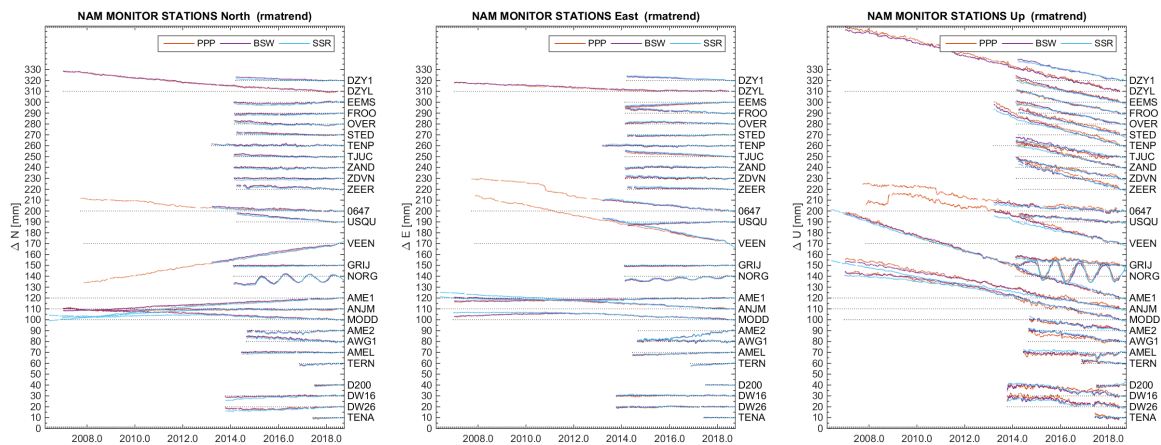
Figure 8.8: Final time series for the NAM monitoring stations, using the 21 day moving average of the trend plus residuals, with common modes removed, and after a reference frame correction for the BSW and PPP solutions: North (left), East (middle) and Up (right). For NORG the harmonic component is added.
