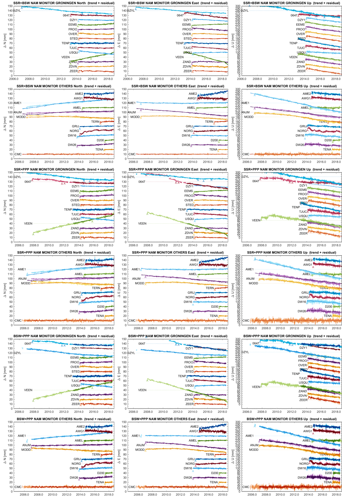
Figure 6.2: Trend plus residuals for the NAM monitoring stations. Two solutions are plotted on top of each other: SSR-BSW (top), SSR-PPP (middle) and BSW-PPP (bottom). The first solution is in a darker color. The time series labeled CMC is the common mode correction that is applied. Antenna changes are marked by a letter “A” and other steps by a “Λ”.
