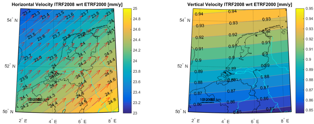
Figure 7.11: Nominal station velocity in ITRF2008 with respect to ETRF2000. The horizontal velocities are shown in the plot on the left, the vertical velocities are shown in the plot on the right.
