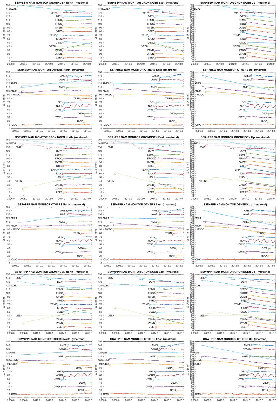
Figure 8.2: Trend plus residuals for the NAM monitoring stations after reference frame correction for the BSW and PPP solutions, smoothed using a 21 day moving average filter. Two solutions are plotted on top of each other: SSR-BSW (top), SSR-PPP (middle) and BSW-PPP (bottom). The first solution is in a darker color. The time series labeled CMC is the common mode correction that is applied. Antenna changes are marked by a letter “A” and other steps by a “Λ”. For NORG the harmonic component is added, see the text.
