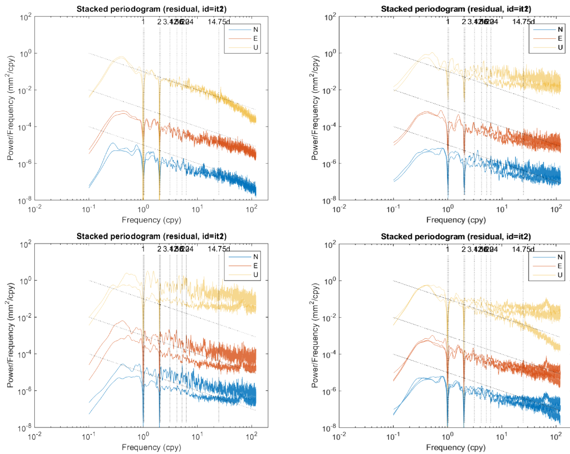
Figure 6.8: Periodograms for the first and second iteration, overlayed on each other, for the SSR solution (top left), the BSW solution (top right) and PPP solution (bottom left). The plot on the bottom right shows the periodograms for the SSR, BSW and PPP solutions overlayed on each other for the second iteration. The plots for the N, E and U component are offset; the slanted dotted lines represent the same power levels.
