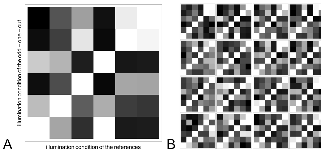
Figure 5. Reaction times for all 30 combinations of illumination conditions. (A) Averaged over all 16 participants. (B) Individual data. Illumination conditions are ordered in the same way as in Figure 4. Black means shortest reaction time; white means longest reaction time.
