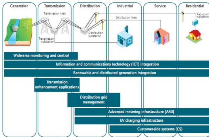
Figure 7: ICT application domains in the Smart Grid. (Source: IEA 2011).
