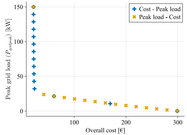
FIGURE 2. Impact of the objective order on the Pareto-front.
