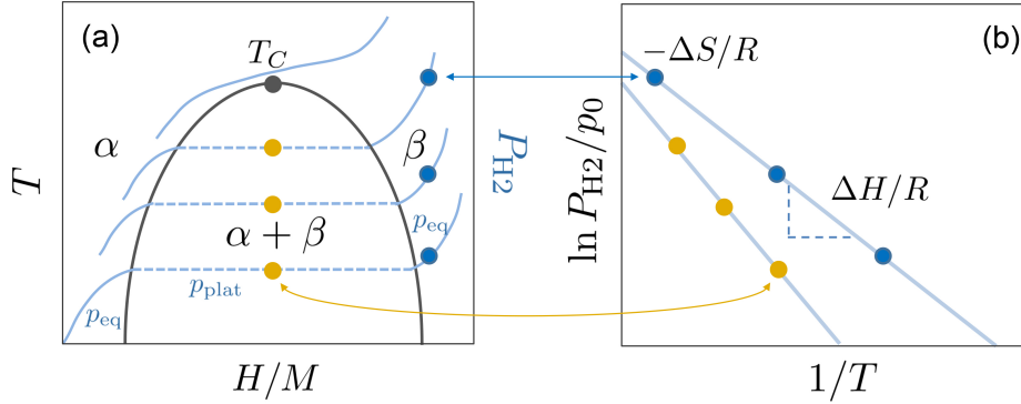
Fig. 3. (Color online) Temperature T and hydrogen-to-metal H/M ratio phase diagram of a typical metal hydride and examples of Pressure-Concentration-Isotherms (PCIs). The \alpha -phase is a diluted solid solution in which hydrogen is typically present in low concentrations. The \beta -phase is the high hydrogen concentration hydride phase that coexists at intermediate H/M with the \alpha -phase. Above the critical temperature T_C , no phase-coexistence (and corresponding first-order phase transition) occurs and only a \alpha -phase exists as an extended solid solution phase. The blue lines and the right axis indicate PCIs. At low and high H/M , the equilibrium pressure p_{\text{eq}} is at a given temperature monotonically increasing in H/M . In the region of phase coexistence, a plateau is seen at the plateau pressure p_{\text{plat}} , which shifts with increasing temperature to higher pressures. (b) Example of a Van 't Hoff plot that can be used to obtain the enthalpy \Delta H and entropy \Delta S_0 . By plotting the natural logarithm of the normalized equilibrium pressure at a given H/M ratio as a function of the inverse temperature, \Delta H and \Delta S_0 may, according to Van 't Hoff's equation (eq. 1), be obtained from the slope and intercept of a linear fit through the points, respectively.
