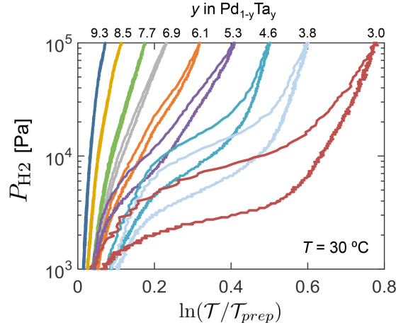
Fig. 6. (Color online) Pressure-Transmission-Isotherms (PTIs) of \text{Pd}_{1-y}\text{Ta}_y films measured at T = 30\text{ }^\circ\text{C} during the fifth hydrogen absorption and desorption cycle. The white-light transmission \mathcal{T} was measured relative to that of the as-prepared film \mathcal{T}_{prep} . For lower Ta concentrations hysteresis between hydrogen absorption and desorption is observed whereas at higher Ta concentrations the hysteresis disappears. The concentration of Ta in the alloy (atomic %) is indicated at the top of the corresponding isotherms. Data adapted from Westerwaal et al. (2012). 50)
