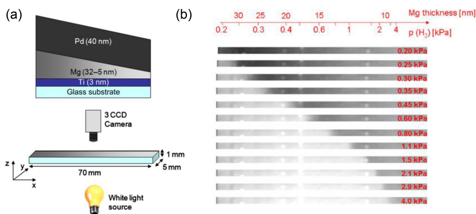
Fig. 7. (Color online) (a) Design of an eye-readable hydrogen sensor based on a Pd-capped Mg thin film with a varying Mg thickness. The sample consists of a wedge of Mg with varying thickness along the x-direction. The Mg wedge is sandwiched between a 40 nm Pd-capping layer and a 3 nm Ti-adhesion layer deposited on a 70 \times 5 \times 1 \text{ mm}^3 glass substrate. The white light optical transmission is measured with a 3CCD camera. (b) Images of the sample when it was exposed to different increasing partial hydrogen pressures of P_{\text{H}_2} = 12 - 4,000 \text{ Pa} at room temperature. Mg has a metal-to-insulator transition when it hydrogenates to \text{MgH}_2 , thus becoming highly transparent upon hydrogenation. The sensor makes use of the profound thickness dependence of the plateau pressure of Mg thin films, which ensures that the metal-to-insulator transition occurs at different pressures. The Mg layer thickness and hydrogenation pressure are reported at the top. This figure is reproduced from Rev. 53) with modifications. © [2010] Elsevier.
