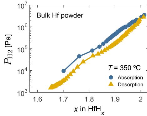
Fig. 11. (Color online) Pressure-Composition-Isotherm (PCI) of bulk powder Hf measured during the second exposure to hydrogen at T = 350\text{ }^{\circ}\text{C} . The 3.3 g Hf powder sample (sponge) was located inside a stainless steel tube which was first evacuated for 20 min. Subsequently, the pressure inside the tube was increased to P_{\text{H}_2} = 2\text{ MPa} at T = 350\text{ }^{\circ}\text{C} using hydrogen gas of 7N purity. Afterwards, the tube was evacuated for 3 h at T = 650\text{ }^{\circ}\text{C} to dehydrogenate. The PCI was measured using the volumetric method.
