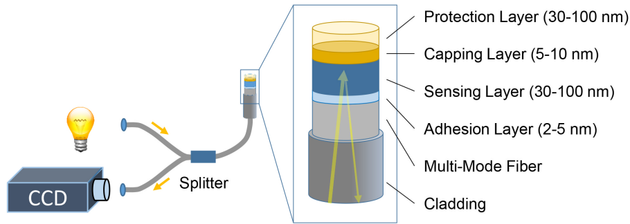
Fig. 2. (Color online) Schematic representation of a micro-mirror optical hydrogen sensor. The light, originating from the light source, is coupled into the fiber and transported to the tip of the optical fiber sensor. The light is partially reflected by the layer stack deposited on the tip of the fiber (see inset) and then passed back through the fiber and the splitter. The signal is subsequently measured by a photodetector as e.g. a charge-coupled device (CCD). Upon a change in hydrogen pressure, the hydrogenation of the sensing layer (30-100 nm) changes, which in turn results in a change of the optical properties and thus the amount of light reflected by the layer stack and detected by a photodetector. The sensing layer is cleaved to the substrate by a 3-5 nm adhesion layer that is often made of Ti. A capping layer (typically Pd or a Pd-based alloy) is used to prevent oxidation of the sensing layer and to catalyze the hydrogen adsorption. This 5-10 nm capping layer is coated with protective polymeric layers as e.g. PTFE and PMMA to protect the Pd layer from being poisoned by harmful chemical species and to further enhance the kinetics of the sensor. Some hydrogen sensors integrate the sensing and capping layer by using a Pd-based alloy (see §3). The figure is not to scale.
