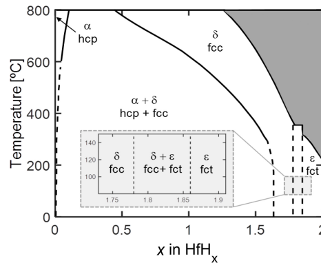
Fig. 10. Phase diagram for bulk hafnium-hydrogen after data from Mintz. 61) \alpha , \delta and \epsilon indicate the hexagonal closed packed (hcp), face centered cubic (fcc) and face centered tetragonal (fct) phase. The shaded area indicates the region of the phase diagram where the hydride formation pressure exceeds 0.1 MPa in bulk. The inset shows a more detailed phase diagram for 1.72 \leq x \leq 1.92 . Although at first sight the phase diagram makes Hf look unsuited for hydrogen sensing applications due to the first-order phase transitions, Hf can be used to hysteresis-free detect hydrogen. The \alpha \rightarrow \delta is irreversible under normal conditions and the \delta \rightarrow \epsilon transition is coherent in nature for thin films. This figure is reproduced from Rev. 43) with modifications. © [2019] Elsevier.
