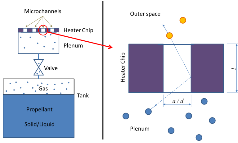
Fig. 1. Schematic of the LPM and its working principle.
