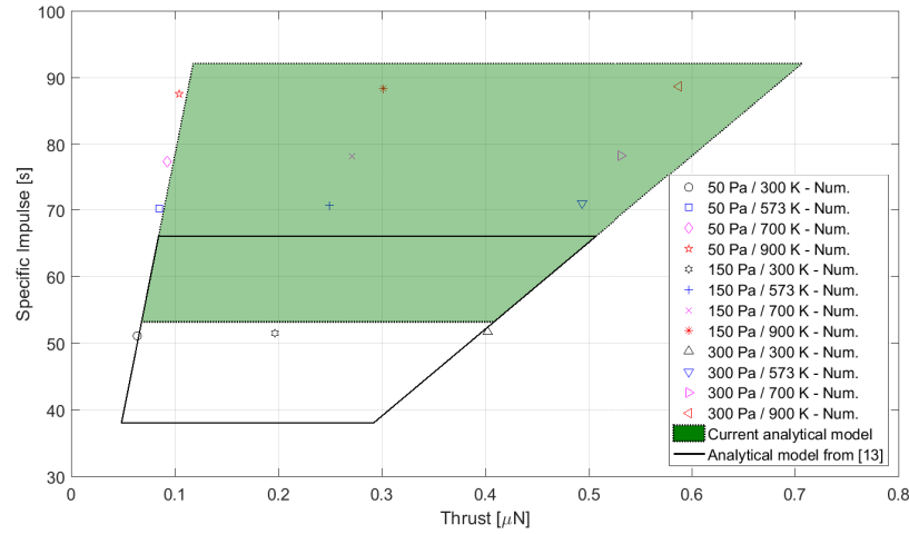
Fig. 3. Thrust versus Specific Impulse for different values of the plenum pressure ranging from 50 to 300 Pa and wall temperature ranging from 300 to 900 K. Comparison between the numerical results presented in [22], the analytical model proposed in [13] and the current analytical model for a single microchannel using Nitrogen with aspect ratio of 5 and plenum temperature of 300 K.
