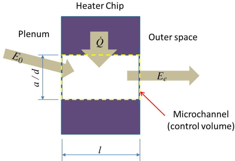
Fig. 2. Balance of the energy inside of the microchannel where E_0 is the energy which gets in the control volume, E_e is the energy which gets out the control volume and \dot{Q} is the heat transferred to the gas inside the control volume.
