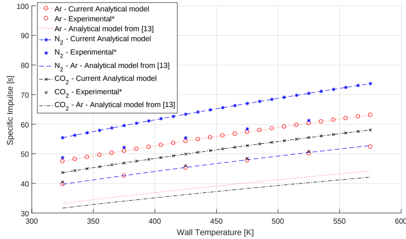
Fig. 6. Specific impulse as a function of T_w for different propellants and constant mass flow rate. *The experimental results were plotted from the fit equations presented in [13].
