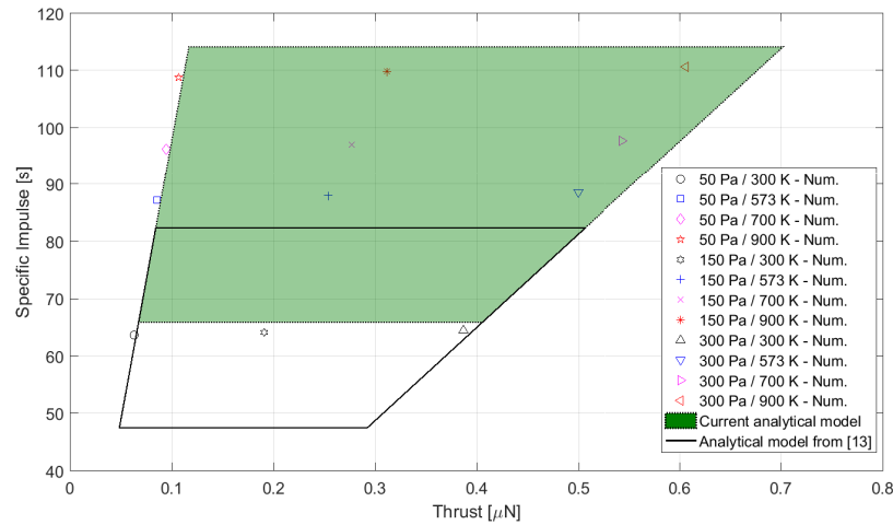
Fig. 4. Thrust versus Specific Impulse for different values of the plenum pressure ranging from 50 to 300 Pa and wall temperature ranging from 300 to 900 K. Comparison between the numerical results presented in [23], the analytical model proposed in [13] and the current analytical model for a single microchannel using Water with aspect ratio of 5 and plenum temperature of 300 K.
