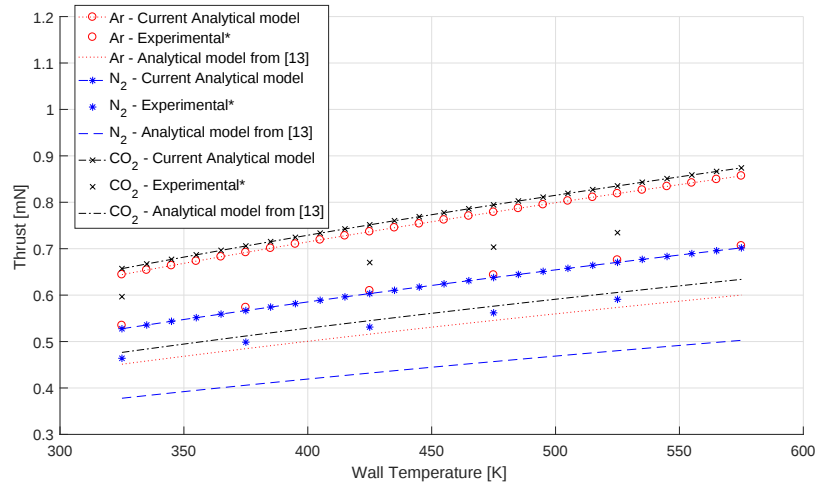
Fig. 5. Thrust as a function of T_w for different propellants and constant mass flow rate. *The experimental results were plotted from the fit equations presented in [13].
