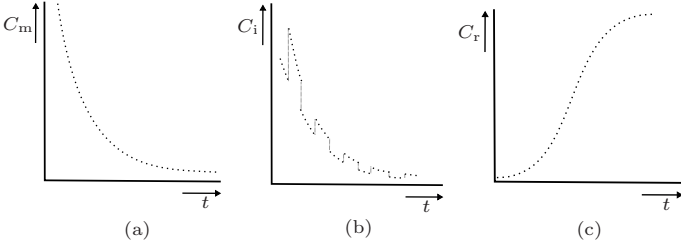
Figure 4: Example relations between the different cost components and the time of maintenance. (a) life-time averaged direct maintenance costs; (b) lifetime-averaged indirect maintenance costs; (c) costs related to risk.
