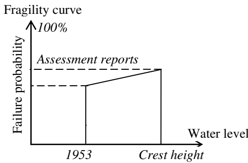
Figure 8. Conceptual example of macro-stability fragility curve for the Hollandsche IJssel
