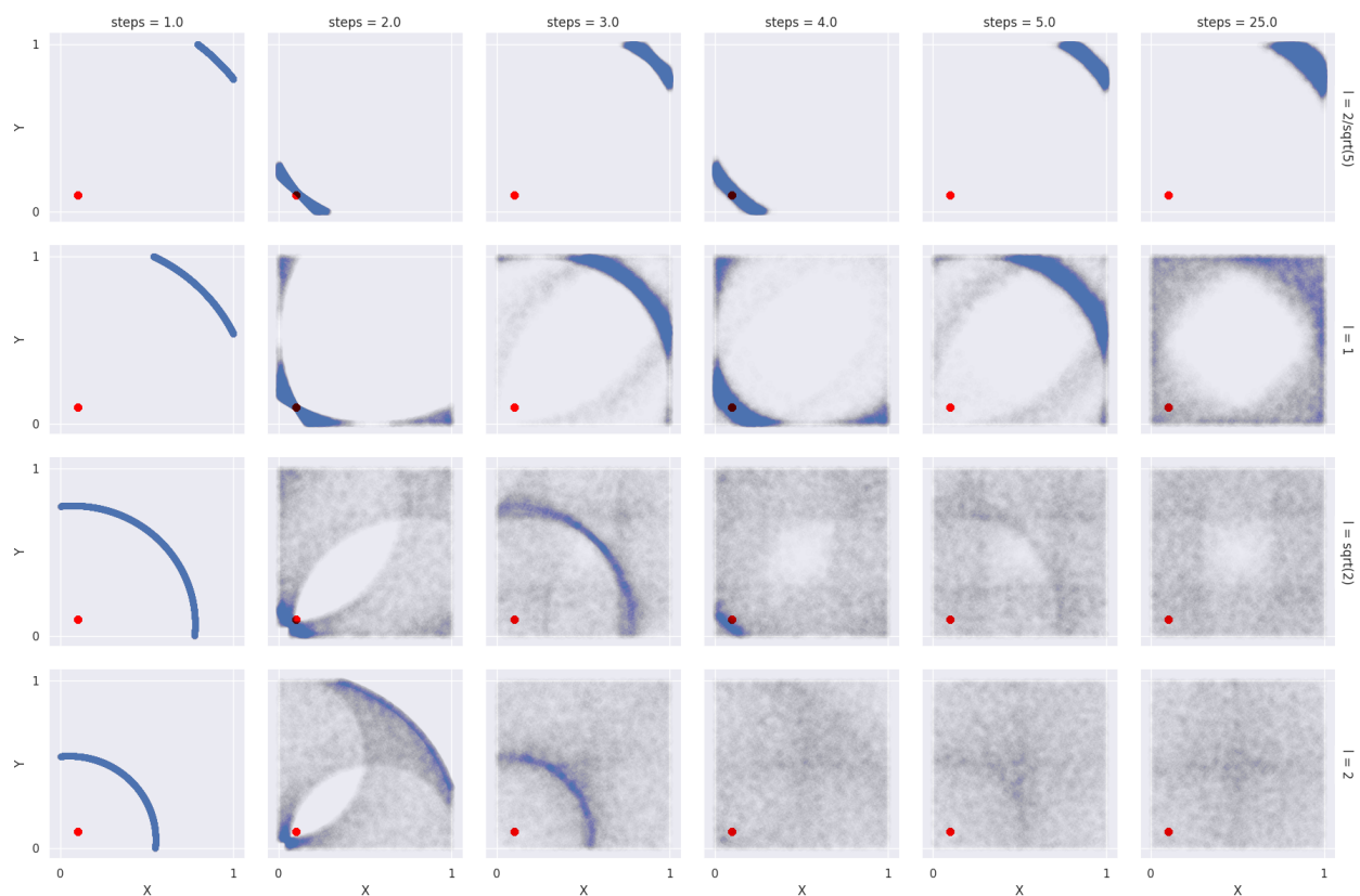
Figure 4: The distribution of the location after a small number of steps (columns, s = 1, 2, 3, 4, 5, 25 ) in different size squares C^2(l) (rows, l = 2/\sqrt{5}, 1, \sqrt{(2)}, 2 ). Each distribution is estimated using 20000 independent Monte-Carlo simulations of the process, starting in the point (0.1, 0.1) (red). The squares are all scaled to size one, so that the ‘unit’ steps are of different sizes.
