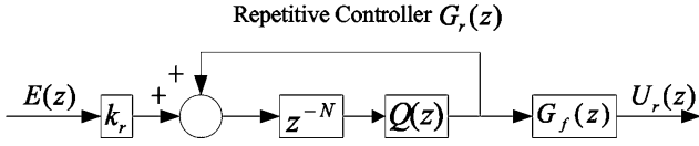
Fig. 2. Repetitive controller.
