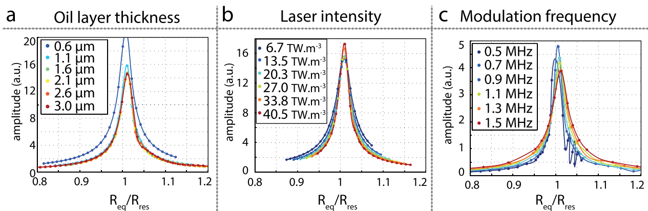
FIG. 7. (Color online) Scaled resonance curves for the finite difference model. (a) Scaled resonance curves at 1 MHz for a heat deposition of 27 \text{ TW/m}^3 with an oil layer thickness varying from 0.6 \mu\text{m} to 3 \mu\text{m} . (b) Scaled resonance curves at 1 MHz for an oil layer thickness of 1 \mu\text{m} and for a heat deposition ranging from 6.7 \text{ TW/m}^3 to 40.5 \text{ TW/m}^3 . (c) Scaled resonance curves for a heat deposition of 27 \text{ TW/m}^3 and an oil layer thickness of 1 \mu\text{m} , and for a frequency ranging from 0.5 to 1.5 \text{ MHz} .
