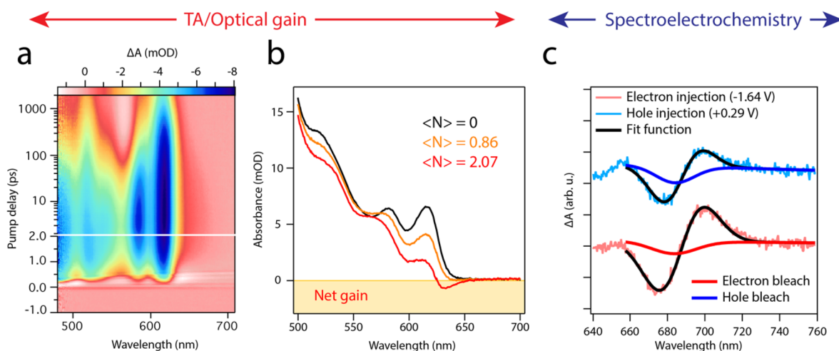
Figure 6. Additional spectroscopic evidence of hole contribution to the BE-bleach. (a) High-fluence TA color map of the CdSe/CdS/ZnS QDs, excited at 400 nm with a fluence of 6.54 \times 10^{14} photons/cm 2 per pulse, showing a maximum of the BE-bleach 4.5 ps after photoexcitation. (b) Comparison between the excited-state absorption spectrum ( A_0 + \Delta A ), obtained from the differential absorbance shown in panel a at 4.5 ps, and the steady state absorption ( A_0 , black), clearly showing the presence of optical gain at \langle N \rangle = 2.07 excitons/QD. (c) Spectroelectrochemical measurement on a film of CdTe QDs, showing the differential absorption spectrum of the sample at reducing potentials (electron injection, red curve) and oxidizing potentials (hole injection, blue curve, offset for clarity). The bleach amplitude was extracted from a fit of the signal with a Gaussian and a derivative-like feature, due to the presence of a Stark shift induced by localized charges. 49
