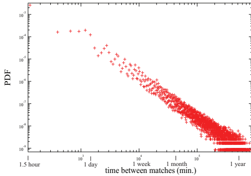
Fig. 2: Probability density of the time between consecutive matches for each player in the DotAlicious dataset.
