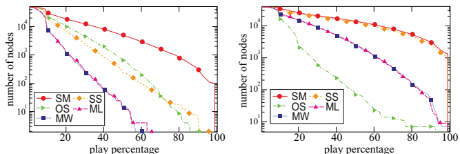
Fig. 4: Number of nodes in the network as a function of the play percentage for Dota-League (left) and DotAlicious (right).
