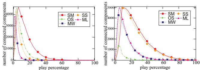
Fig. 7: Number of strongly connected components with PP mapping for Dota-League (left) and DotAlicious (right).
