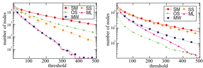
Fig. 3: Number of nodes in the network as a function of the threshold for Dota-League (left) and DotAlicious (right).
