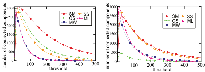
Fig. 6: Number of connected components for Dota-League (left) and DotAlicious (right).
