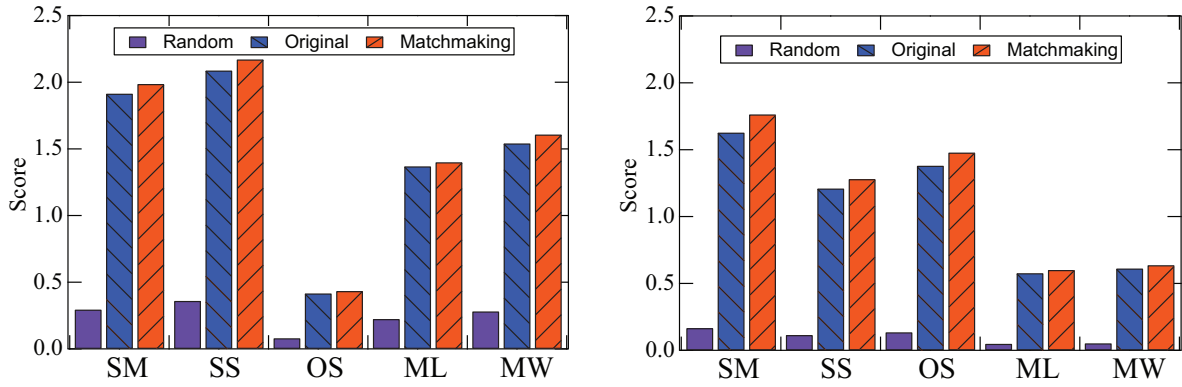
Fig. 8: Average match scores when performing matchmaking for DotAlicious (left) and Dota-League (right).
