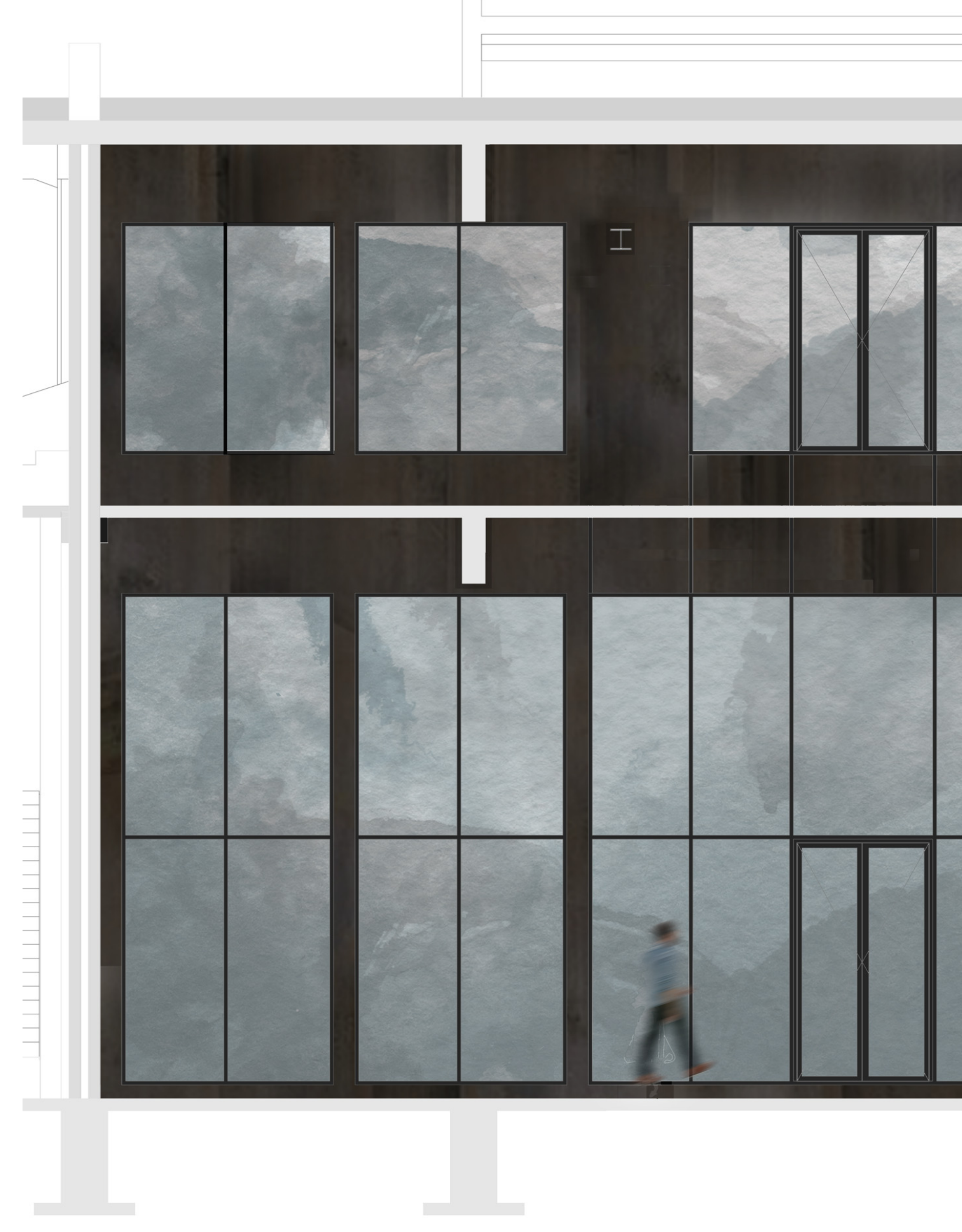
FACADE FRAGMENT ELEVATION 1/50
