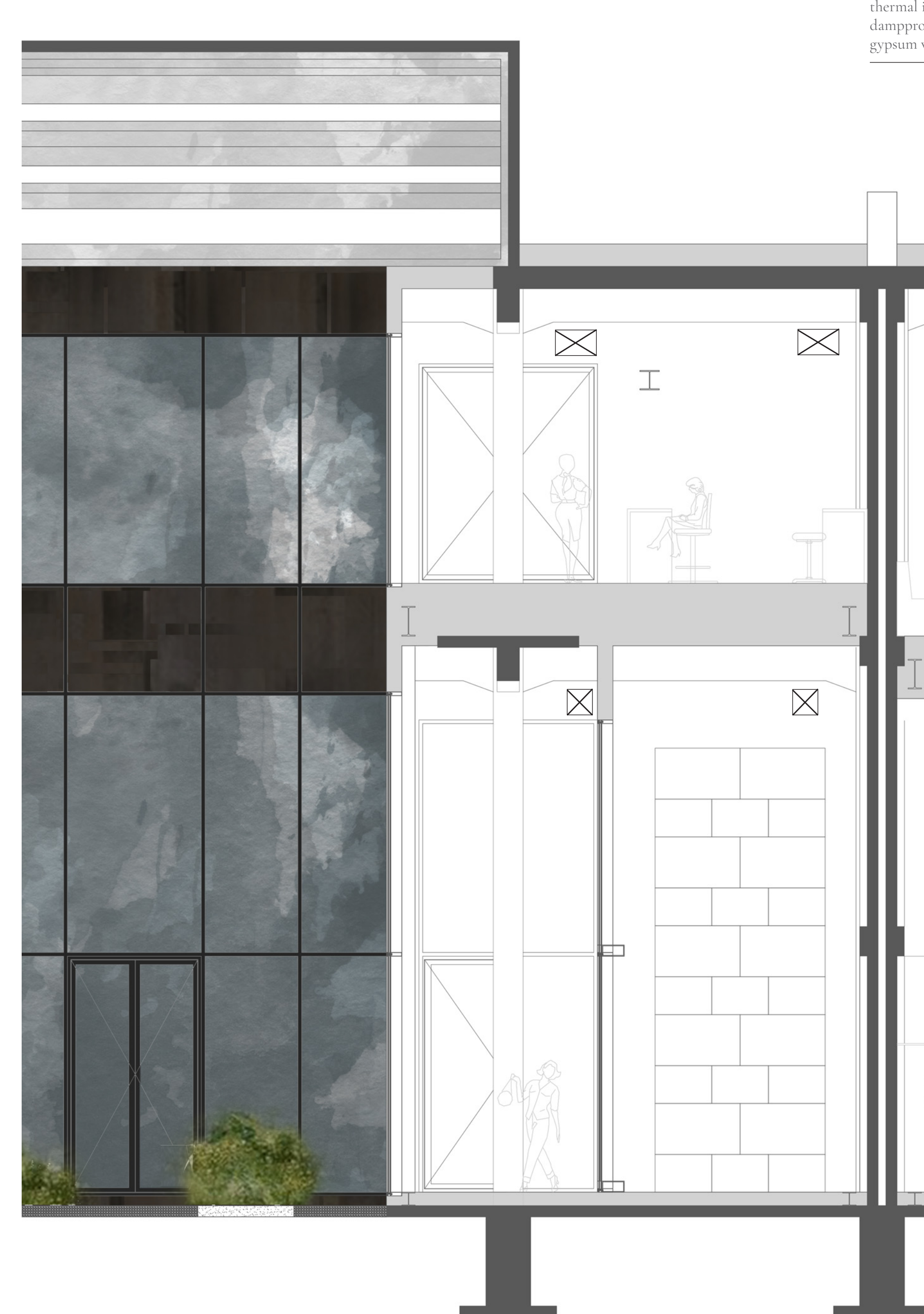
FACADE FRAGMENT ELEVATION 1/50
