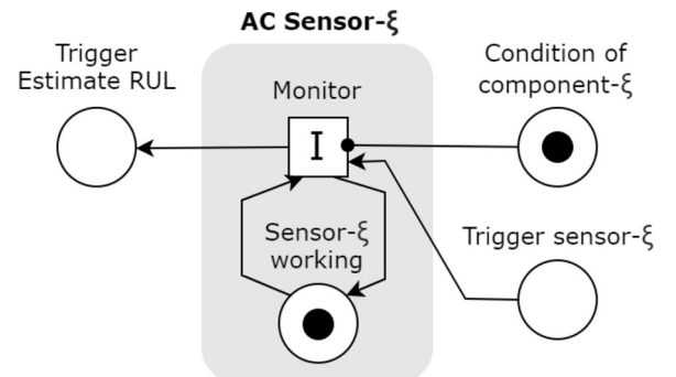
Fig. 8. LPN: Sensor- \xi of the agent AC.
