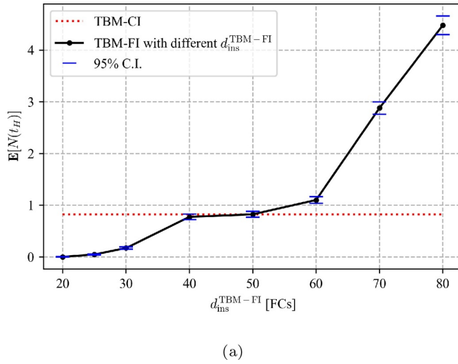
Fig. 23. Expected number of the brake-related safety incidents and expected total number of tasks under TBM-FI with different d_{\text{ins}}^{\text{TBM-FI}} .
