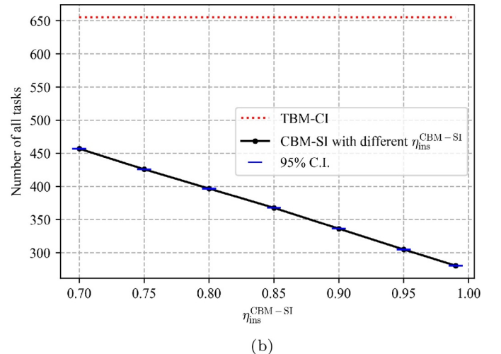
Fig. 24. Expected number of the brake-related safety incidents and expected total number of tasks under CBM-SI with different \eta_{\text{ins}}^{\text{CBM-SI}} .
