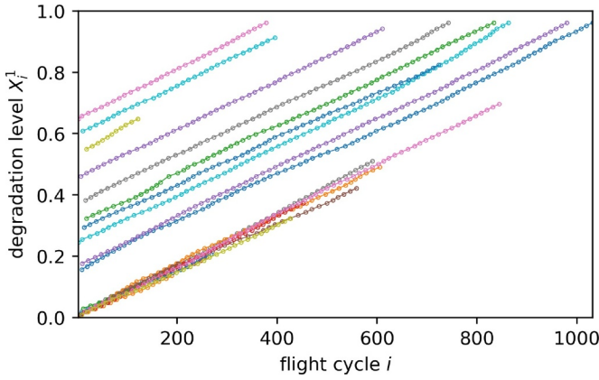
Fig. 20. Degradation level data of the aircraft brake-1.
