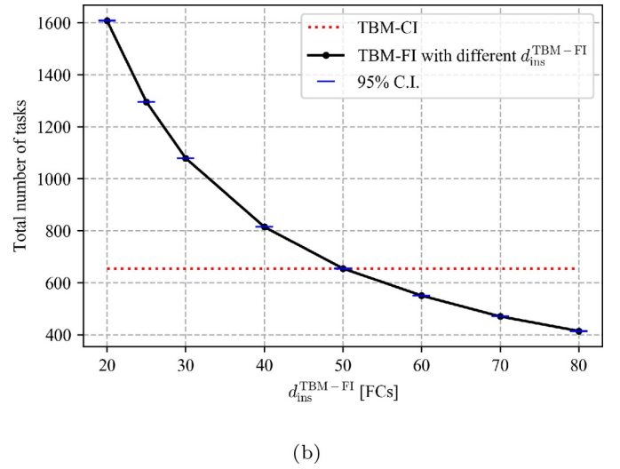
Fig. 23. Expected number of the brake-related safety incidents and expected total number of tasks under TBM-FI with different d_{\text{ins}}^{\text{TBM-FI}} .
