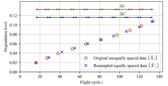
Fig. 21. Degradation process data example – unequally spaced data points \tilde{X}_i , and equally spaced data points \tilde{X}'_i , after resampling.
