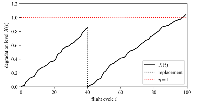
Fig. 16. A realisation of the degradation process following eq. (12).
