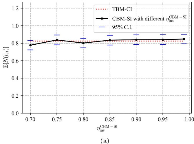
Fig. 24. Expected number of the brake-related safety incidents and expected total number of tasks under CBM-SI with different \eta_{\text{ins}}^{\text{CBM-SI}} .
