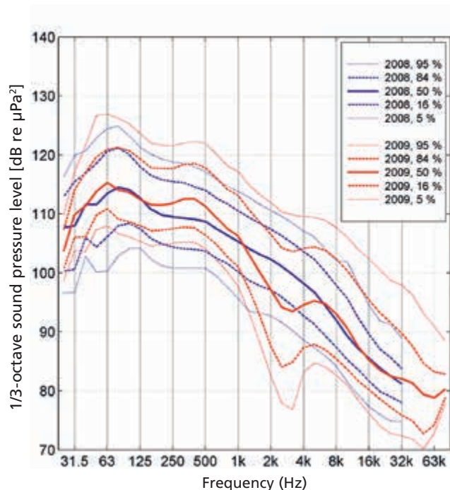
Figure 5. Statistic N percent exceedance levels of the measured sound pressure levels (SPL) per one-third-octave band at a fixed station in the area between the borrow area and the Maasvlakte 2 construction area in 2008 (blue lines) and 2009 (red lines). The dip in the 2009 curves at 3 kHz may be the result of the night-time presence of large numbers of small fish with a swim bladder (see de Jong et al. 2010).
