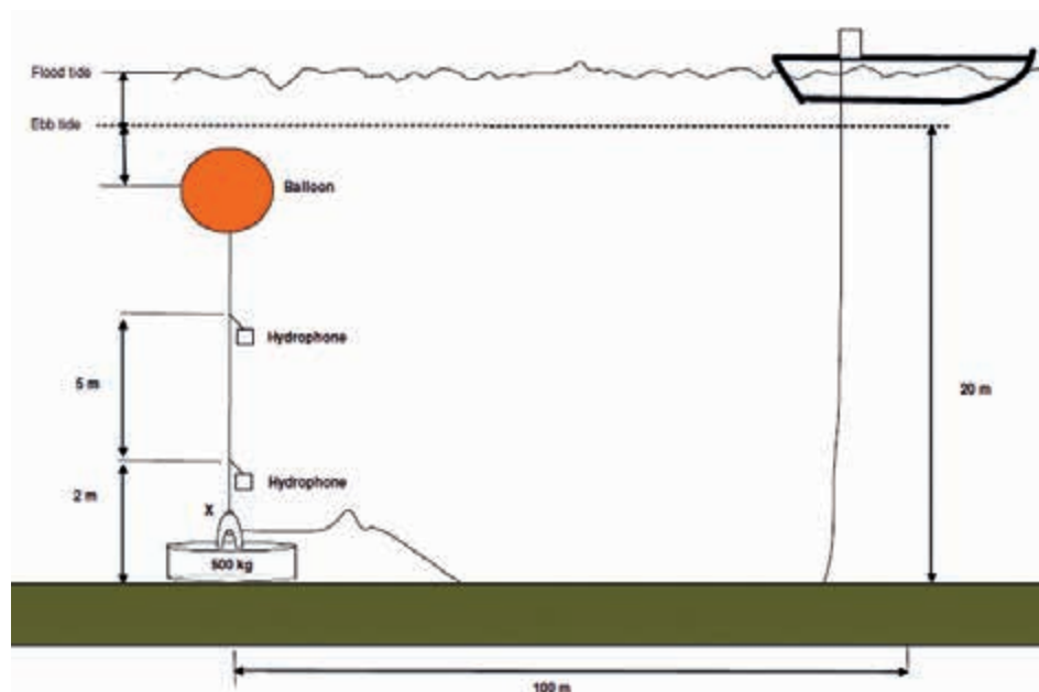
Figure 2. Schematic representation of the fixed monitoring set-up at location Z during the baseline measurements in 2008.
