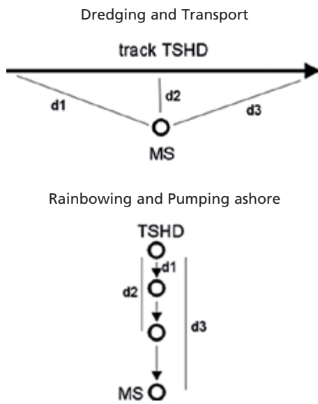
Figure 6. Above, procedures for measuring underwater radiated sound of dredgers during various operations (de Jong et al. , 2010). For a reliable estimation of the source level, measurements with one or more hydrophones are carried out at several distances ( d_1 , d_2 , d_3 ). MS = Measurement station.
