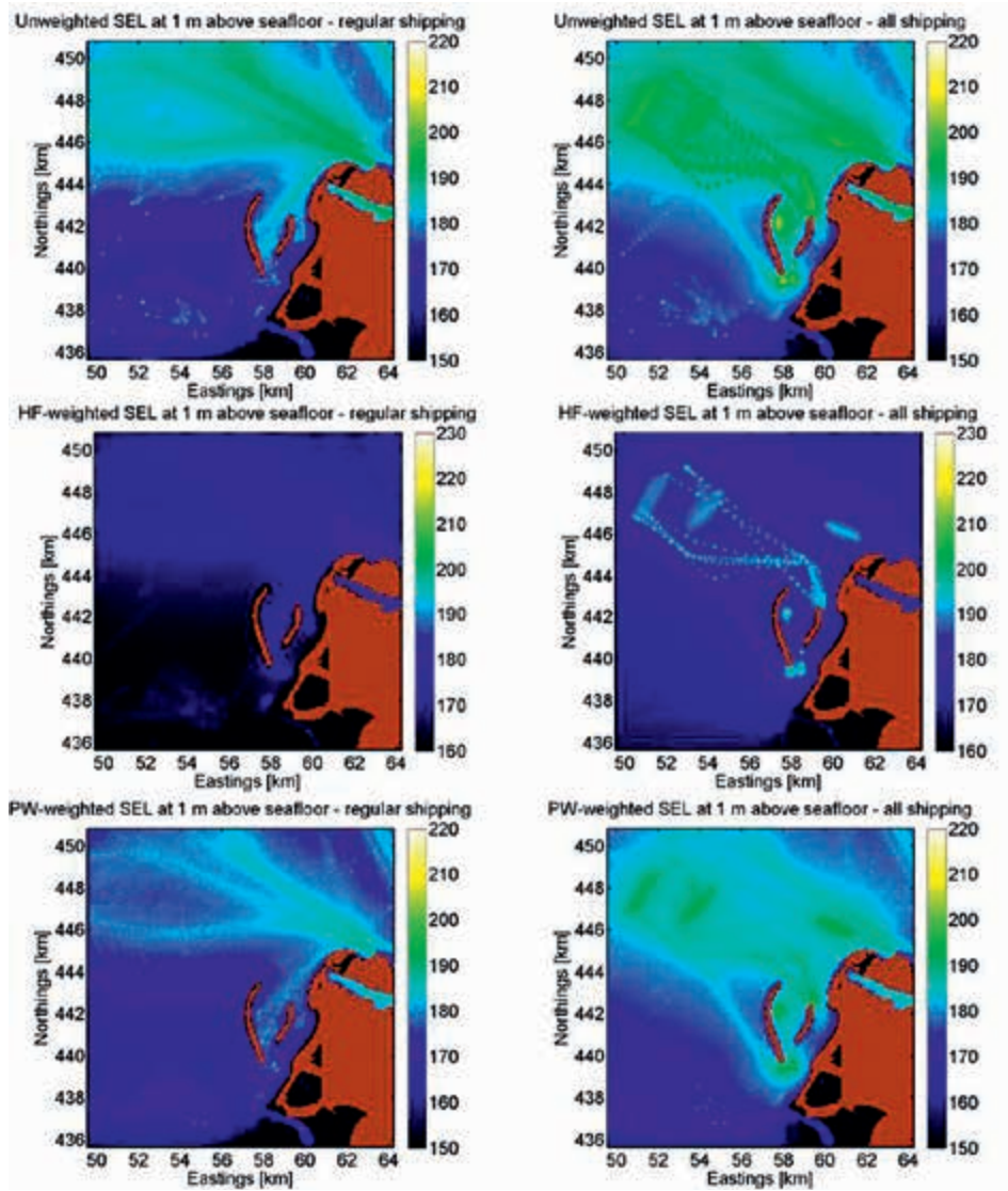
Figure 10. Sound maps generated by regular shipping (left) and regular shipping + dredgers (right) at a depth of 1 m above the seafloor. The figure shows the cumulative broadband sound exposure level (dB Re 1 µPa²s) for a period of 24 hours: non-weighted (top, representative for fish), M-weighted for “high frequency cetaceans” (centre, representative for harbour porpoise) and M-weighted for “pinnipeds in water” (bottom, representative for seals).
