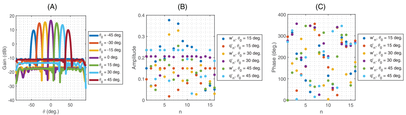
FIGURE 4 Results of optimization of excitation coefficients ( w_n^{fs}, q_n^{fs} ) in the 16-element linear array at 9 GHz for \pm 45 degree scanning with 15-degree steps when q_{\max} = 1 : (A) realized gains for horizontal polarization, (B) excitation amplitudes, (C) excitation phases [Color figure can be viewed at wileyonlinelibrary.com ]
