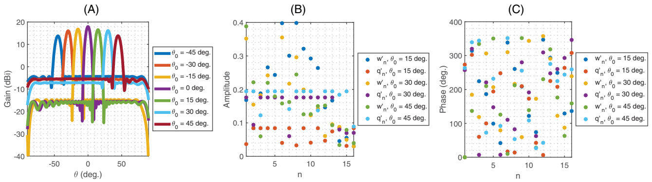
FIGURE 3 Results of optimization of excitation coefficients ( w_n^{fs}, q_n^{fs} ) in the 16-element linear array at 9 GHz for \pm 45 degree scanning with 15-degree steps when q_{\max} = 0.5 : (A) realized gains for horizontal polarization, (B) excitation amplitudes, (C) excitation phases [Color figure can be viewed at wileyonlinelibrary.com ]
