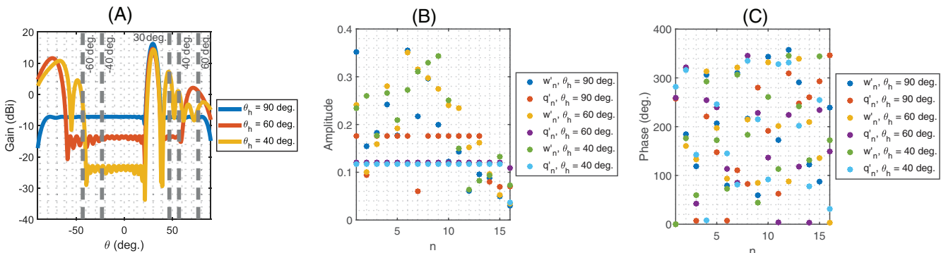
FIGURE 5 Results of optimization of excitation coefficients ( w_n^{fs}, q_n^{fs} ) in the 16-element linear array at 9 GHz for 30 degree scanning when \theta_h = [90 \ 60 \ 40] degrees, q_{\max} = 0.5 : (A) realized gains for horizontal polarization, (B) excitation amplitudes, (C) excitation phases [Color figure can be viewed at wileyonlinelibrary.com ]
