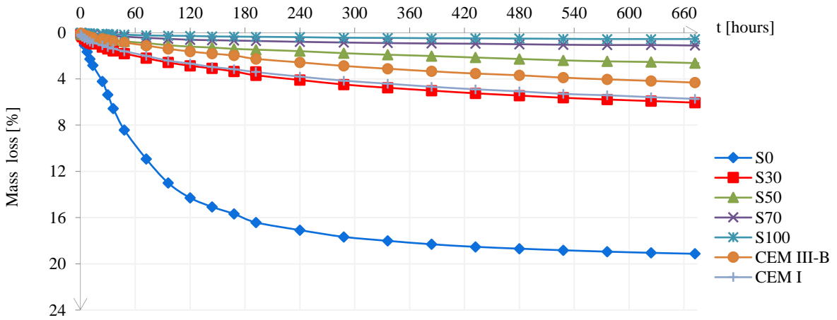
Fig. 3. Unsealed samples first 28 days; mass loss measured from 28 days.
