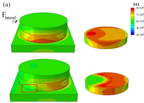
Fig. 8: (a) The stress contour of delamination test with lateral loading at the displacement of 1.5 nm/2.5nm, the right graph is the interface stress distribution of Cu dot; (b) the lateral load-displacement curve and the corresponding damage dissipation energy graph.
