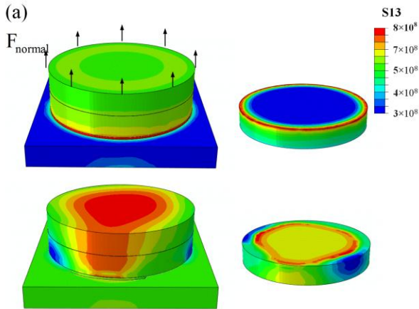
Fig. 9: (a) The stress contour of delamination test with normal loading at the displacement of 0.4 nm/0.7nm, the right graph is the interface stress distribution of Cu dot; (b) the normal load-displacement curve and the corresponding
