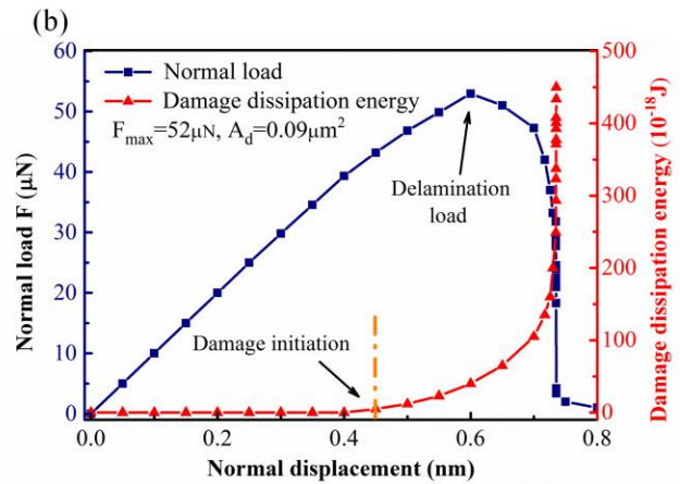
Fig. 9: (a) The stress contour of delamination test with normal loading at the displacement of 0.4 nm/0.7nm, the right graph is the interface stress distribution of Cu dot; (b) the normal load-displacement curve and the corresponding
