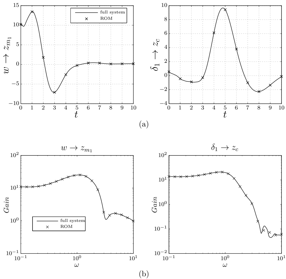
Figure 3. Performance of the reduced order model (ROM) compared with the full system: (a) Impulse response, (b) magnitude frequency response from disturbance w to output z_{m_1} and from input \delta_1 to the controlled output z_c .
