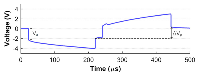
Fig. 14 Measured voltage waveform between the cathode and the anode electrodes for a 1 \text{ mA} stimulation with maximum pulse widths of 200 \mu\text{s} . For this recording one electrode on the array was selected in a monopolar configuration
