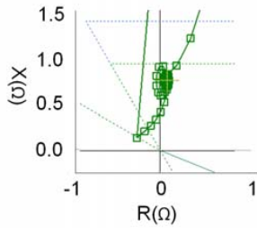
Fig. 6. Manufacturers distance relay performance for phase-to-ground fault with 40 MW generation level with protection zones.
