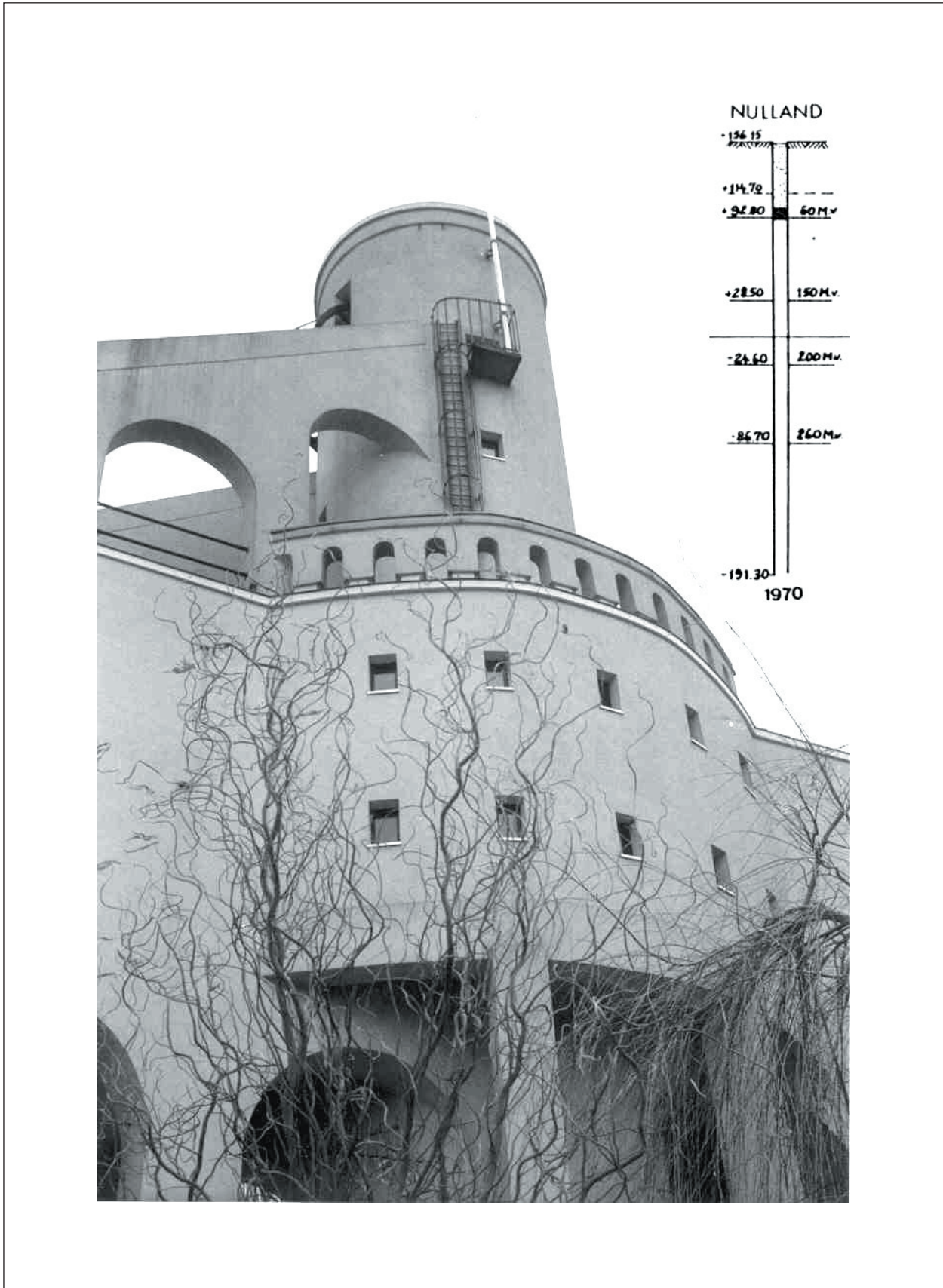
Figure 2. The restored Nulland shaft of the former Domaniale mine (Kerkrade, the Netherlands). At the top, right, a cross section of the shaft with the depths of the former levels. The upper level is filled with a concrete plug at -60 m depth. The closure year was 1970. (Photograph R. van de Laar, 1995)
