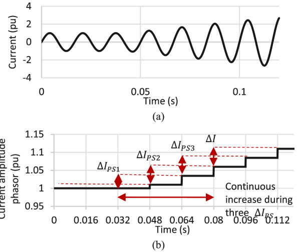
Fig. 3. Stable power swing (a) current signal and, (b) current phasor amplitude in both in pu.
